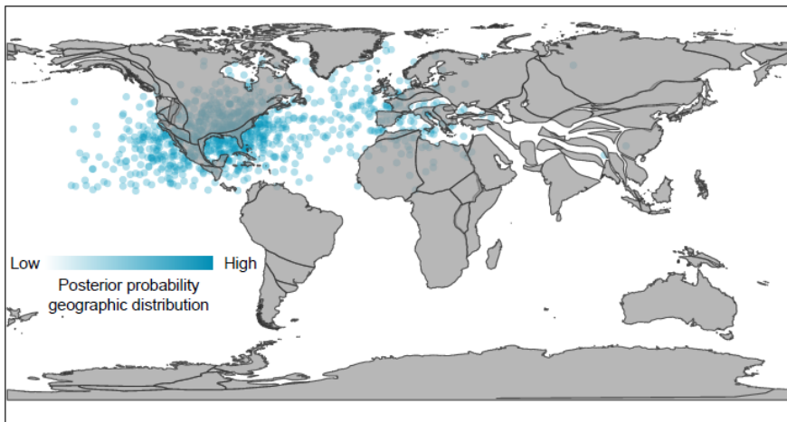
Supplementary Figure 3. Posterior geographic distribution and posterior probability of habitat type for eight phylogenetic nodes. We selected eight random nodes ranging from 111 to 33 Mya. 1 = 78 Mya; 2 = 56 Mya; 3 = 52 Mya; 4 = 41 Mya; 5 = 40 Mya; 6 = 38.8 Mya; 7 = 38.4 Mya; 8 = 36 Mya. a. The posterior coordinates were estimated with Geo model. b. The ancestral habitat type for these eight random nodes was estimated using phylogenetic models for discrete trait evolution.
