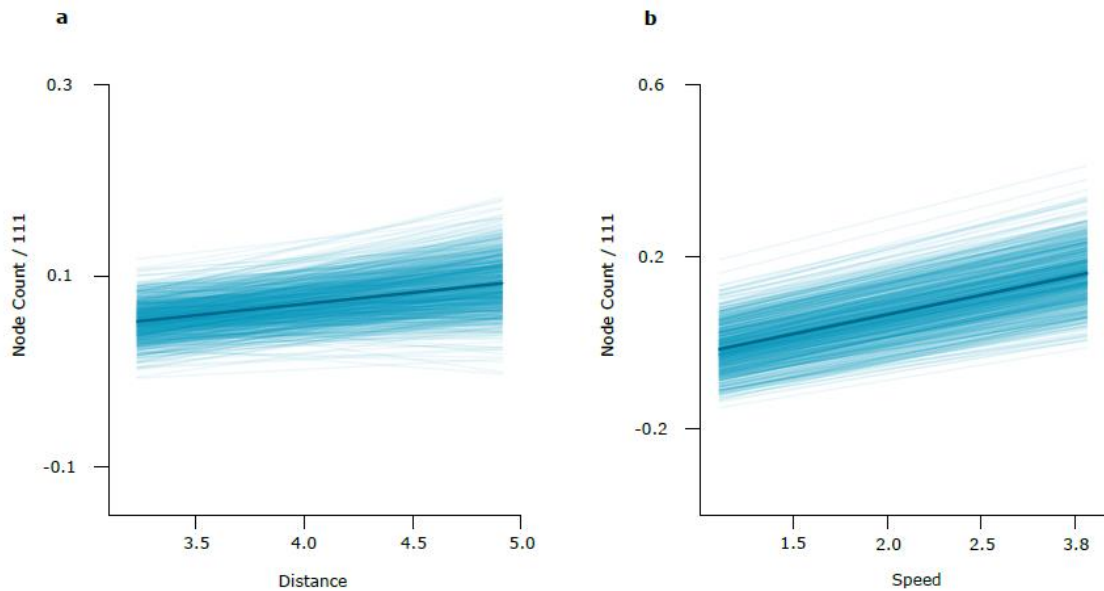
Figure 6. Clupeiformes with lower dispersal abilities have lower probabilities of originate new species. a - b. The Bayesian phylogenetic generalized least squares show that the pathwise distance of movement and the pathwise speed of movement has a positive effect on speciation ( P_{\text{MCMC}} = 0.04 and 0, respectively; n = 157,000 observations sampled from species data). These results support the prediction in Fig. 1g. Lighter lines show the posterior distribution of slopes and dark lines shows the posterior mean slopes. These slopes were estimated while sampling the pathwise distance and speed within species (Methods). Line equation for a and b : y = -0.21 + 0.023(\text{Distance}) + 0.09(\text{Speed}) . The node count values were divided by the tree length after excluding D. clupeoides (111 Myr).
