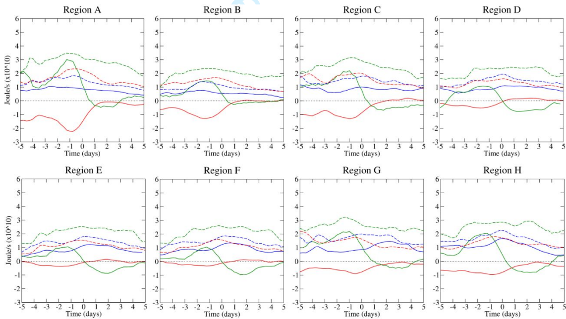
Figure 10 Same as Fig. 5 but for the eight regions defined in Fig. 9. The terms BRC (blue), BRT (red) and AFC (green) are given in solid line with their corresponding standard deviation in dashed line. The number of tracks for each region are: 741 (A), 950 (B), 746 (C), 1042 (D), 1048 (E), 1047 (F), 804 (G) and 611 (G).
