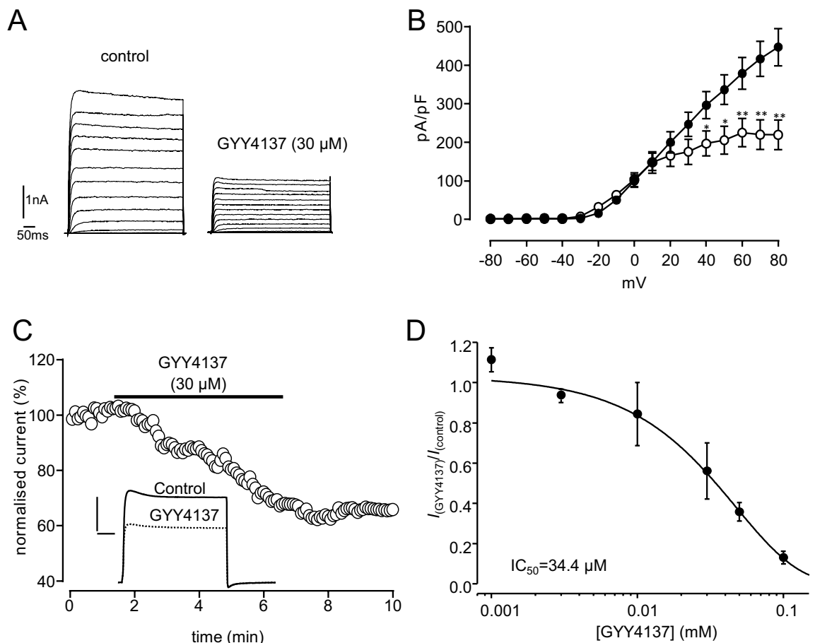
Figure 2. GYY4137 inhibits recombinant Kv2.1. (A) Families of currents evoked in a HEK293 cell stably expressing Kv2.1 before and during exposure to GYY4137 (30 \mu M). Currents were evoked by step-depolarizations, applied up to +80 mV in 10 mV increments from a holding potential of -70 mV. Scale bars apply to both families of currents. (B) Mean ( \pm s.e.m.) current-density versus voltage relationships obtained in 11 cells before (solid circles) and during (open circles) exposure to GYY4137 (30 \mu M). Significance: * P < 0.05; ** P < 0.01 as compared with controls. (C) Example time-series plot illustrating normalized current amplitudes evoked by step-depolarizations in a Kv2.1-expressing HEK293 cell. For the period indicated by the horizontal bar, GYY4137 (30 \mu M) was applied via the perfusate, indicated by horizontal bar, followed by washout. Inset shows example currents under the different experimental conditions scale bars: 2 nA (vertical) and 10 ms (horizontal). (D) Mean ( \pm s.e.m., each point taken from 3 to 5 cells) concentration-response relationship fitted to sigmoidal Boltzmann function illustrating the effects of GYY4137 on Kv2.1. Inhibition was determined using currents evoked by step-depolarizations from -70 to +50 mV.
