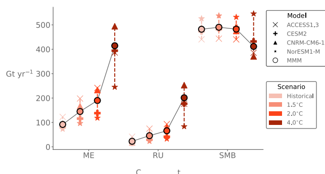
Figure 2. Plot showing mean total melt (ME), runoff (RU) and surface mass balance (SMB), in \text{Gt yr}^{-1} , for Antarctic ice shelves during the historical period (1980–2009) and for global mean warming scenarios of 1.5°C, 2°C, and 4°C above pre-industrial levels in all GCM-forced MAR simulations. Colors indicate the scenario, and each model is plotted with a unique marker. The MMM is indicated with outlined circle and dashed vertical lines indicate the inter-model spread. GCM, global climate models; MAR, Modèle Atmosphérique Régional; MMM, multi-model mean.
