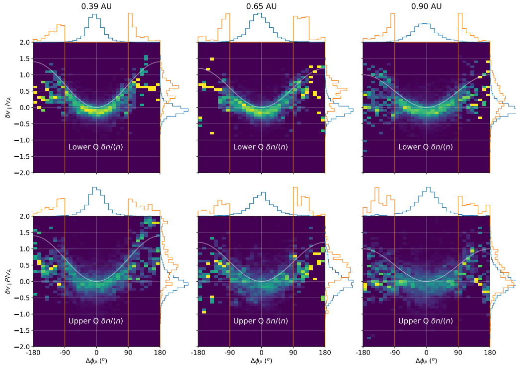
Figure 8. 2-dimensional histograms of \delta v_{\parallel} / v_A against \Delta\phi_P for three radial distance bins in the same format as the top row of Figure 2. The top (bottom) row of plots include data within the lower (upper) quartile of |\delta n / \langle n \rangle| within each distance bin. Above each panel, the blue histogram shows the distribution of \Delta\phi_P for all samples included in the respective 2-dimensional histogram, while the orange histogram shows the distribution of \Delta\phi_P for included inverted HMF samples only. The orange and blue histograms are normalised independently. To the right of each panel, normalised histograms show the distribution of \delta v_{\parallel} / v_A for combined uninverted and inverted HMF samples (blue line) and for inverted samples only (orange line) included in the respective 2-dimensional histogram.
