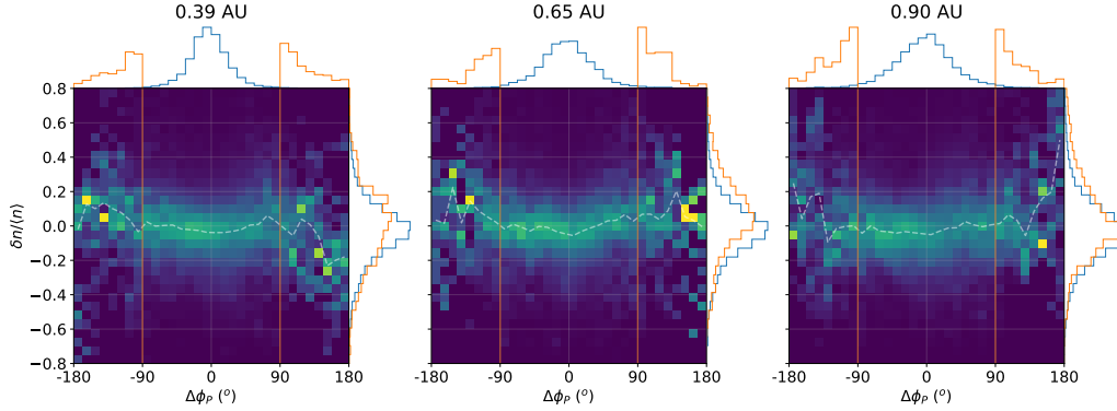
Figure 6. 2-dimensional histograms of \delta n / \langle n \rangle = (n - \langle n \rangle) / \langle n \rangle against \Delta\phi_P for three radial distance bins. \langle n \rangle is calculated over 12 hours. A dashed white line shows the median value in each column of \Delta\phi_P . The figure is in the same format as the top row of Figure 2. Above each panel, the blue histogram shows the distribution of \Delta\phi_P for all samples in a given distance bin, while the orange histogram shows the distribution of \Delta\phi_P for inverted HMF samples only. The orange and blue histograms are normalised independently. To the right of each panel, normalised histograms show the distribution of \delta n / \langle n \rangle for combined uninverted and inverted HMF samples (blue line) and for inverted samples only (orange line).
