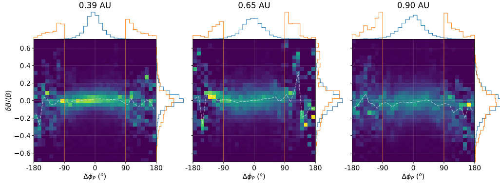
Figure 7. 2-dimensional histograms of \delta B / \langle B \rangle = (B - \langle B \rangle) / \langle B \rangle against \Delta\phi_P for three radial distance bins. \langle B \rangle is calculated over 12 hours. A dashed white line shows the median value in each column of \Delta\phi_P . The figure is in the same format as the top row of Figure 2. Above each panel, the blue histogram shows the distribution of \Delta\phi_P for all samples in a given distance bin, while the orange histogram shows the distribution of \Delta\phi_P for inverted HMF samples only. The orange and blue histograms are normalised independently. To the right of each panel, normalised histograms show the distribution of \delta B / \langle B \rangle for uninverted and inverted HMF samples combined (blue line) and for inverted samples only (orange line).
