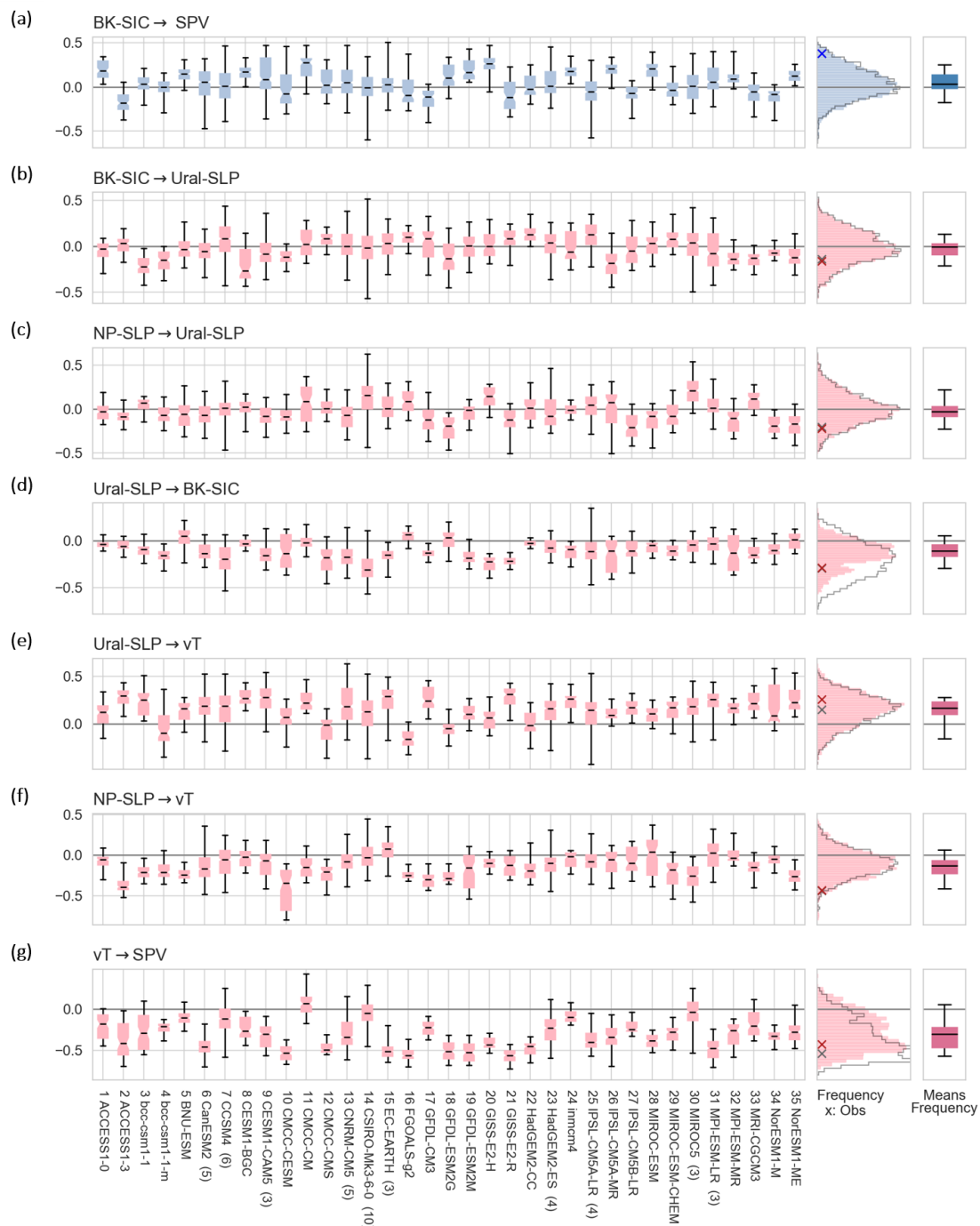
Figure 4. Individual links of Arctic–stratosphere pathway. Links from (a) seasonal-mean BK-SIC (in OND) to SPV (in JFM) and from (b) monthly BK-SIC (in N) to Ural-SLP (in J), (c) NP-SLP (in D) to Ural-SLP (in J), (d) Ural-SLP (in N) to BK-SIC (in D), (e) Ural-SLP (in D) to vT (in J), (f) NP-SLP (in D) to vT (in J), and (g) vT (in J) to SPV (in F). What is shown is the spread in link strength for each model (left panels) and the distribution of all link strengths (middle panels) and of the models' means (right panels). The link strengths are quantified by regressing each variable on their parents (see Fig. 3) for each model over 39-year moving windows from 1900 to 2005 (in total 67 windows) in the historical simulations. Grey contours in the middle panel show the histogram obtained using (unadjusted) regression. The crosses in the middle panel denote the link strength obtained using observations (grey for unadjusted regression and coloured crosses for regressions including all parents). Numbers in brackets after model names on the x axis indicate the number of ensemble members used, with no number meaning that just one member was used. The box and whisker plots thus include different amounts of data (number of ensemble members times the 67 moving windows). The boxes indicate the inter-quartile range, the whiskers represent the upper and lower quartile ranges, and horizontal lines show the median.
