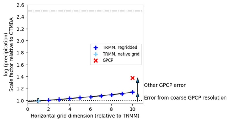
Extended data Figure 1. Effect of low spatial resolution in GPCP satellite observations of \log(\text{seasonal precipitation}) . y-axis: regression gradient in validation against GTMBA rain gauge data (i.e. gradients in Figure 1 for light blue and red symbols). x-axis: horizontal grid dimension relative to TRMM (e.g. the TRMM resolution is 0.25^\circ , ten times smaller than the GPCP resolution of 2.5^\circ , so the red symbol is placed at x=10 ). Dark blue symbols: results when TRMM data is regridded (by area averaging) to coarser grids. The coarser grids are chosen so the grid box edges overlap edges of the native TRMM grid. To give the errors context, the dash-dot line marks the ratio between the largest and smallest model values of k_{\text{qsat}} (2.5). Solid black line is a quadratic least-squares best fit line through the TRMM-based data. The intercept of the TRMM best-fit curve at x=0 (i.e. infinitely fine grid) is very close to the value estimated on the TRMM native grid (light blue symbol), indicating that the TRMM grid is sufficiently fine for comparison with the rain gauge data on seasonal timescales.
