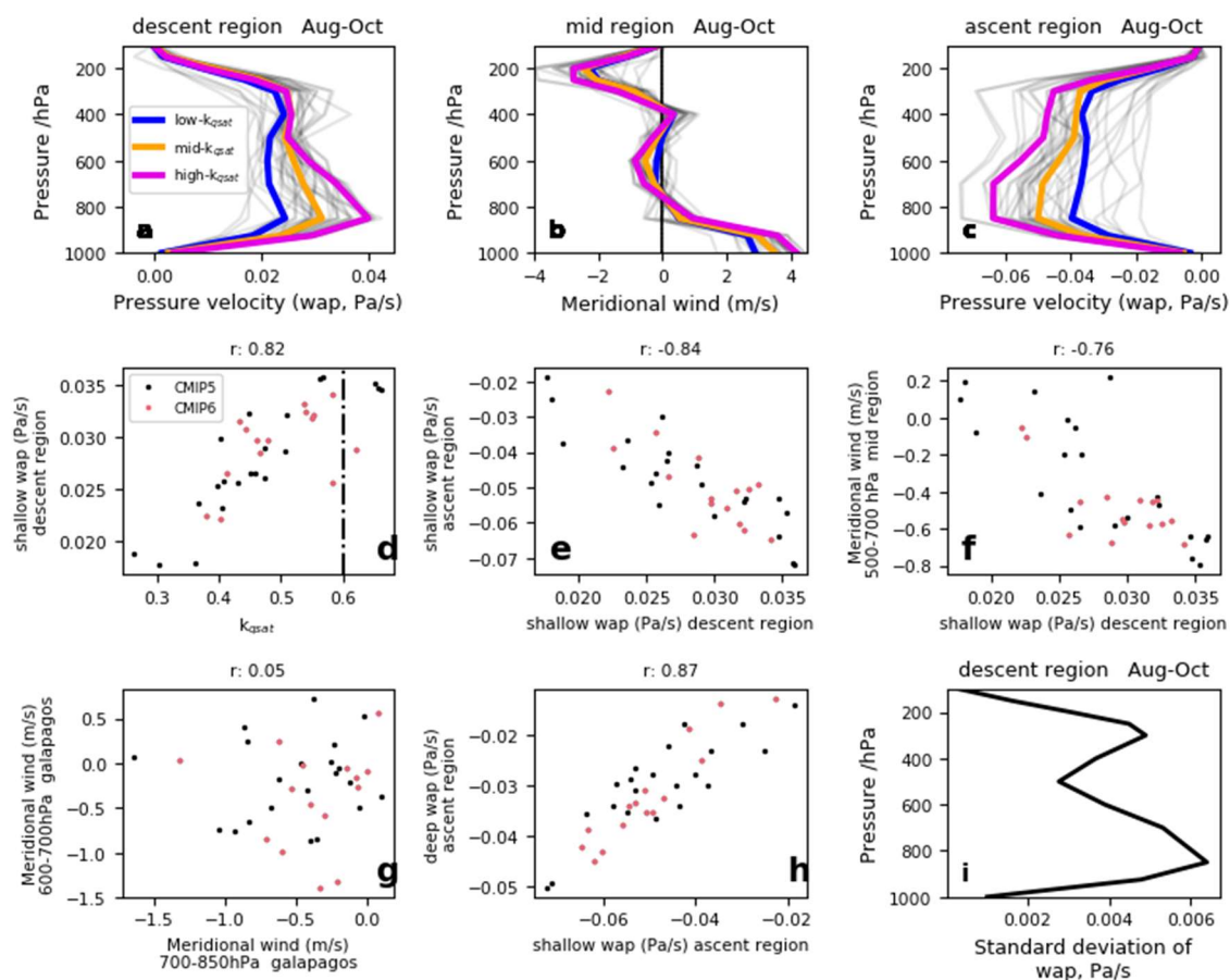
Extended Data Figure 8. Atmospheric circulation measures in CMIP5 and CMIP6 models.
