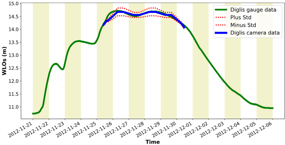
Fig. 5. Water level information extracted from Farson Digital Ltd river camera images at Diglis Lock. The new river-camera-derived water levels are plotted against the nearest river gauge station, Diglis, approximately 274 m from the camera along the river.
