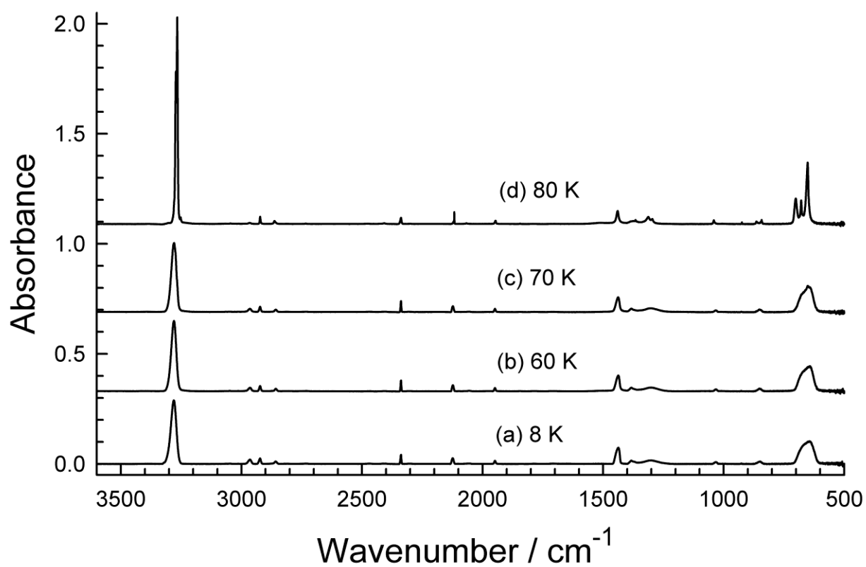
Fig. 10. Mid-IR survey spectra of C_3H_4 deposited at 8 K and warmed to the temperatures indicated. Spectra are offset for clarity.
