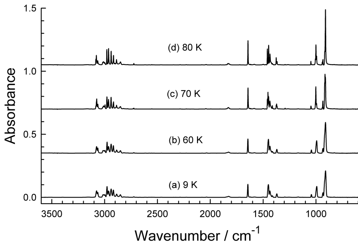
Fig. 5. Mid-IR survey spectra of \text{C}_3\text{H}_6 deposited at 9 K and warmed to the temperatures indicated. Spectra are offset for clarity.
