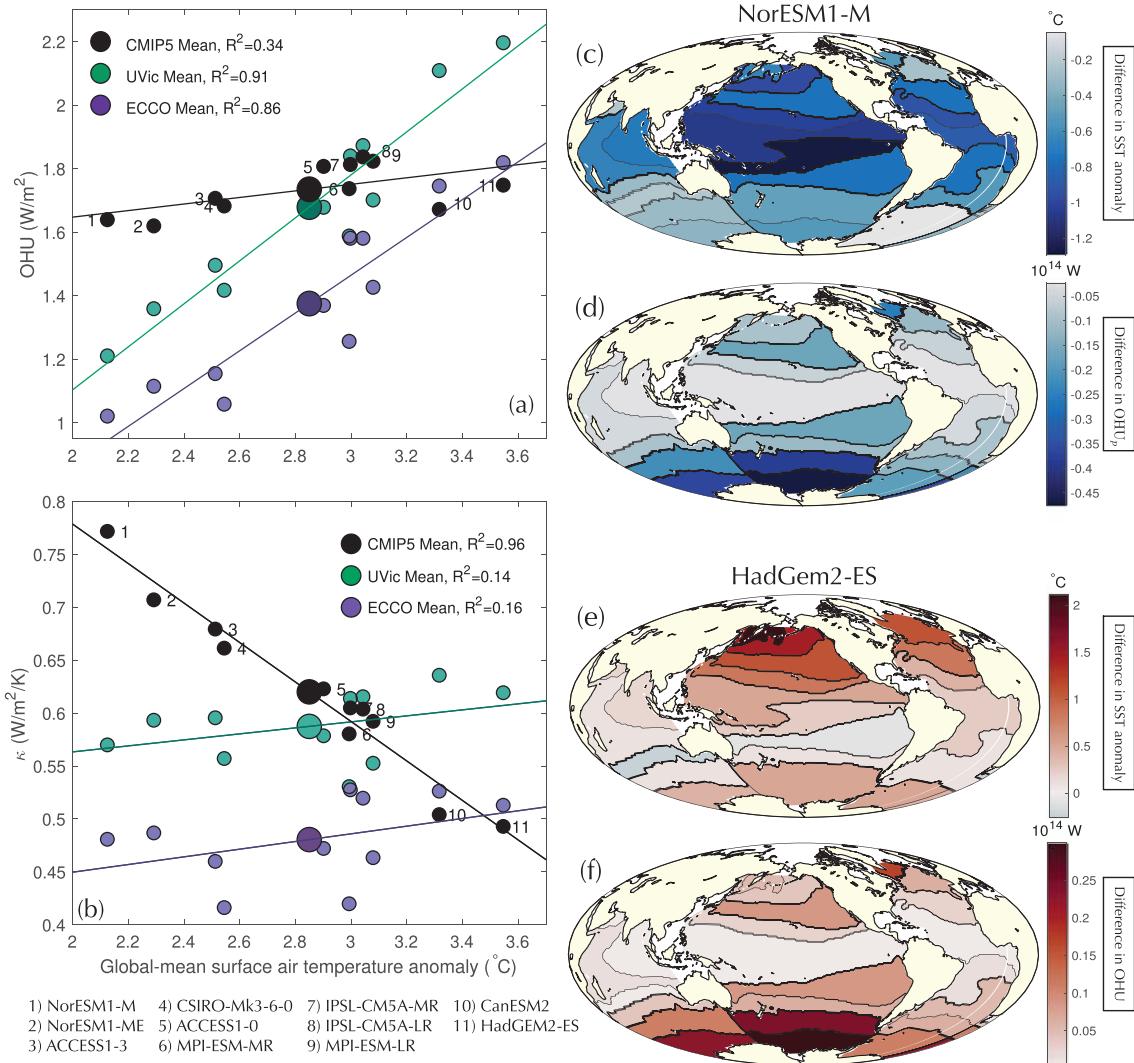
Figure 2. Variations in ocean heat uptake, ocean uptake efficiency, and surface warming between simulations. (a) \overline{\text{OHU}} with global-mean surface air temperature anomaly, \bar{T} , for individual CMIP5 simulations (black). Each simulation's GF counterpart simulation, calculated with UVic (green) and the ECCO (purple), includes only passive heat uptake, \overline{\text{OHU}}_p . The mean value in each ensemble is also included (large circles). (b) \kappa for each CMIP 5 model (black) and (passive) \kappa_p for each GF counterpart simulation (UVic in green and ECCO in purple) with \bar{T} . In both, the ensemble-mean values are shown (large circles). (c) The difference in sea surface warming pattern in the coolest model outlier, NorESM1-M, from the CMIP5 ensemble-mean pattern (i.e., \Delta\text{SST}_c(j, t) - \Delta\text{SST}_o(j, t) , where “o” stands for outlier). (d) The associated anomaly in the total passive heat uptake per patch from the UVic ensemble-average pattern. (e) The same as (c) but for the warmest model outlier, HadGem2-ES; (f) the same as in (d) but for HadGem2-ES. Fields in all panels are averages over years 60–130 of the experiments.
