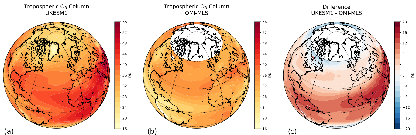
Figure 8. The spatial patterns of tropospheric ozone column (in DU), averaged from 2000–2014 in (a) UKESM1 historical simulations and (b) for satellite observations (OMI-MLS). Panel (c) shows the difference between model and satellite estimates (in DU).
