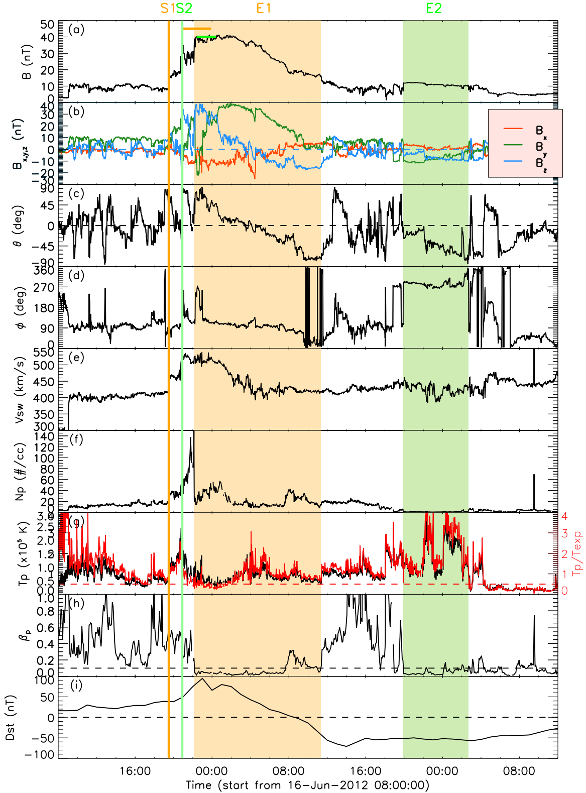
Figure 6. CME measurements at Wind. The panels show from top to bottom (a) the magnetic field strength; (b) the x , y , and z magnetic field components in GCS; (c, d) the elevation \theta and azimuth \phi of field direction in GSE; (e) the solar wind velocity; (f) the proton density; (g) temperature (red, expected temperature from Lopez 1987); (h) proton \beta ; and (i) D_{st} index. The yellow and green vertical lines indicate the arrival of S1 and S2, respectively. The yellow and green shaded regions indicate the intervals of CME-1 and CME-2.
