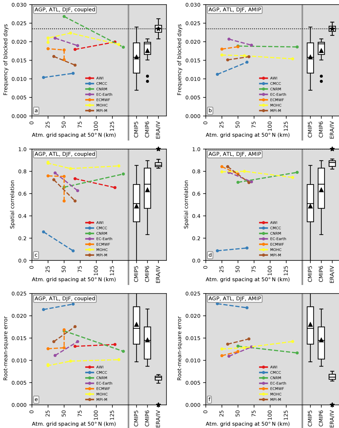
Figure 3. Metrics of blocking performance (a, b – blocking frequency, c, d – spatial correlation, e, f – root-mean-square error) for the AGP index and boreal winter for the ATL domain (50–75° N, –90–90° E). The left-hand side of each panel shows metrics for PRIMAVERA simulations at different grid spacings (resolutions). Box-and-whisker plots (boxplots hereinafter) on the right-hand side show distributions of the metric across CMIP5 and CMIP6 simulations in terms of the median, mean (triangle), and interquartile range (box, IQR = Q3 - Q1 ), with top whiskers extending to the last datum less than Q3 + 1.5 \times IQR and analogously for bottom whiskers. The “*” symbol in the column “ERA/IV” shows the reanalysis estimate, and the boxplot is an estimate of the expected agreement given internal variability (see text).
