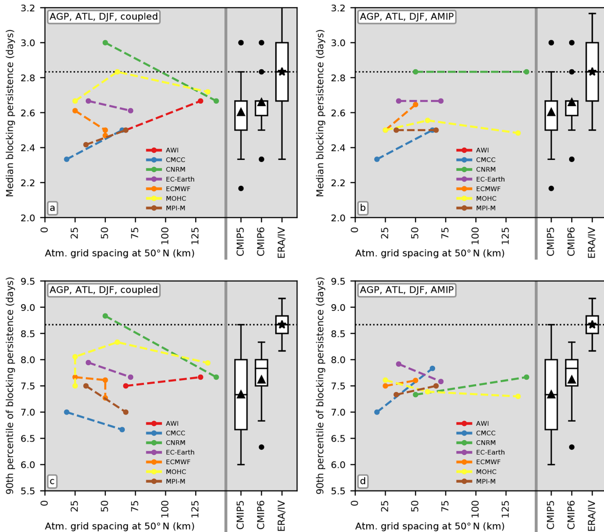
Figure 5. Persistence of blocking events (a, b – median, c, d – 90th percentile) for the AGP index and boreal winter and for the ATL domain (50–75° N, –90–90° E). The left-hand side of each panel shows metrics for PRIMAVERA simulations at different grid spacings (resolutions). Boxplots on the right-hand side show distributions of the persistence metric across CMIP5 and CMIP6 simulations. The “ERA/IV” symbol in the column “ERA/IV” shows the reanalysis estimate, and the boxplot is an estimate of the expected agreement given internal variability (see text).
