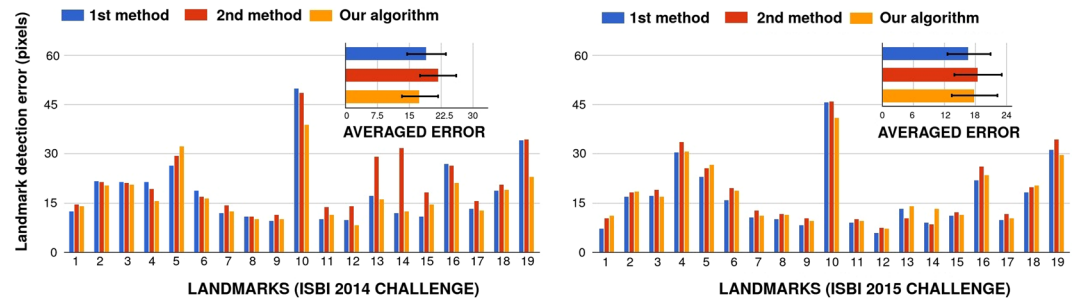
Figure 7. Comparison with 2014 and 2015 ISBI Cephalometric X-Ray Challenge best results.
