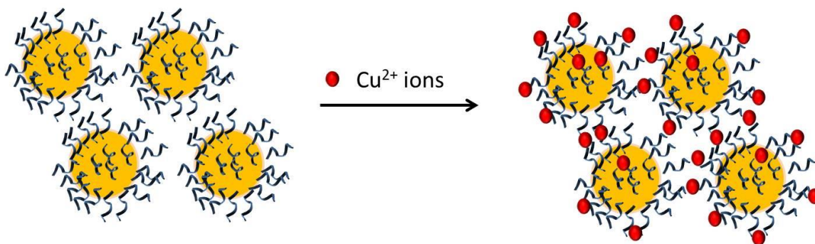
Figure 7. Schematic representation of the Cu 2+ coordination to the AuNP-peptide conjugates.
