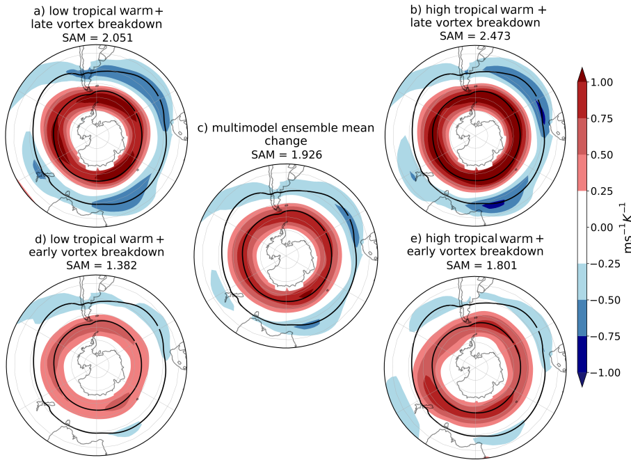
Fig. 8 DJF u_{850} response per degree of warming ( \text{ms}^{-1}\text{K}^{-1} ), meaning that to obtain the response for a global-mean warming of 2^{\circ}\text{C} these values should be multiplied by two. (a),(b),(d),(e) are plausible storylines of climate change related to extreme values of TW and VB delay. (c) shows the MEM u_{850} response. Black contours show the 8 \text{ ms}^{-1} MEM u_{850} in the historical simulations. SAM index ( \text{hPa K}^{-1} ) is computed as the change in the mean climatological SAM
