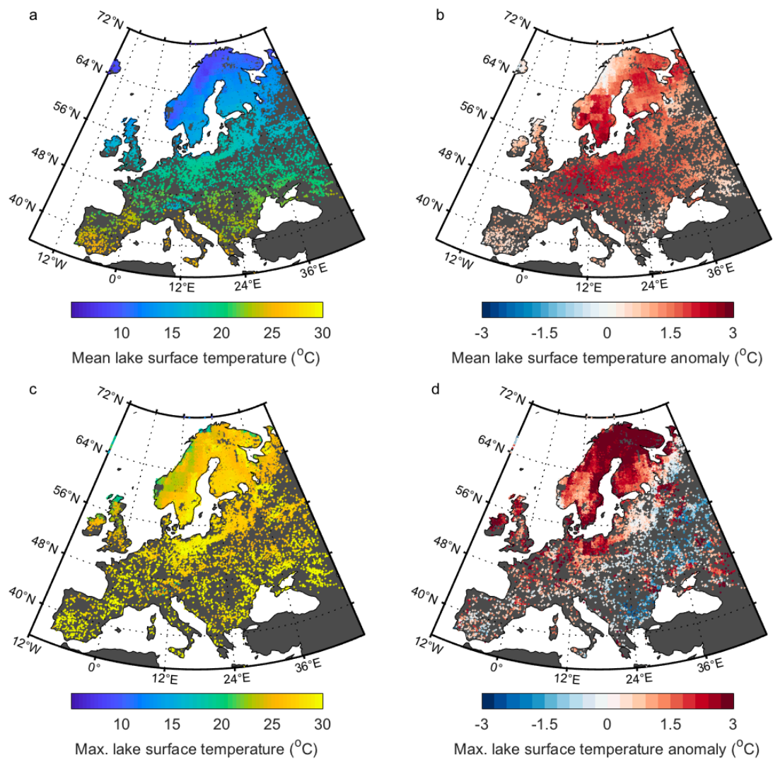
554 Figure 2. Continental-scale variations in May-Oct 2018 (a) mean lake surface water 555 temperature; (b) mean lake surface water temperature anomalies; (c) maximum lake 556 surface water temperature; (d) maximum lake surface water temperature anomalies. 557 Anomalies are shown relative to the 1981-2010 average.
