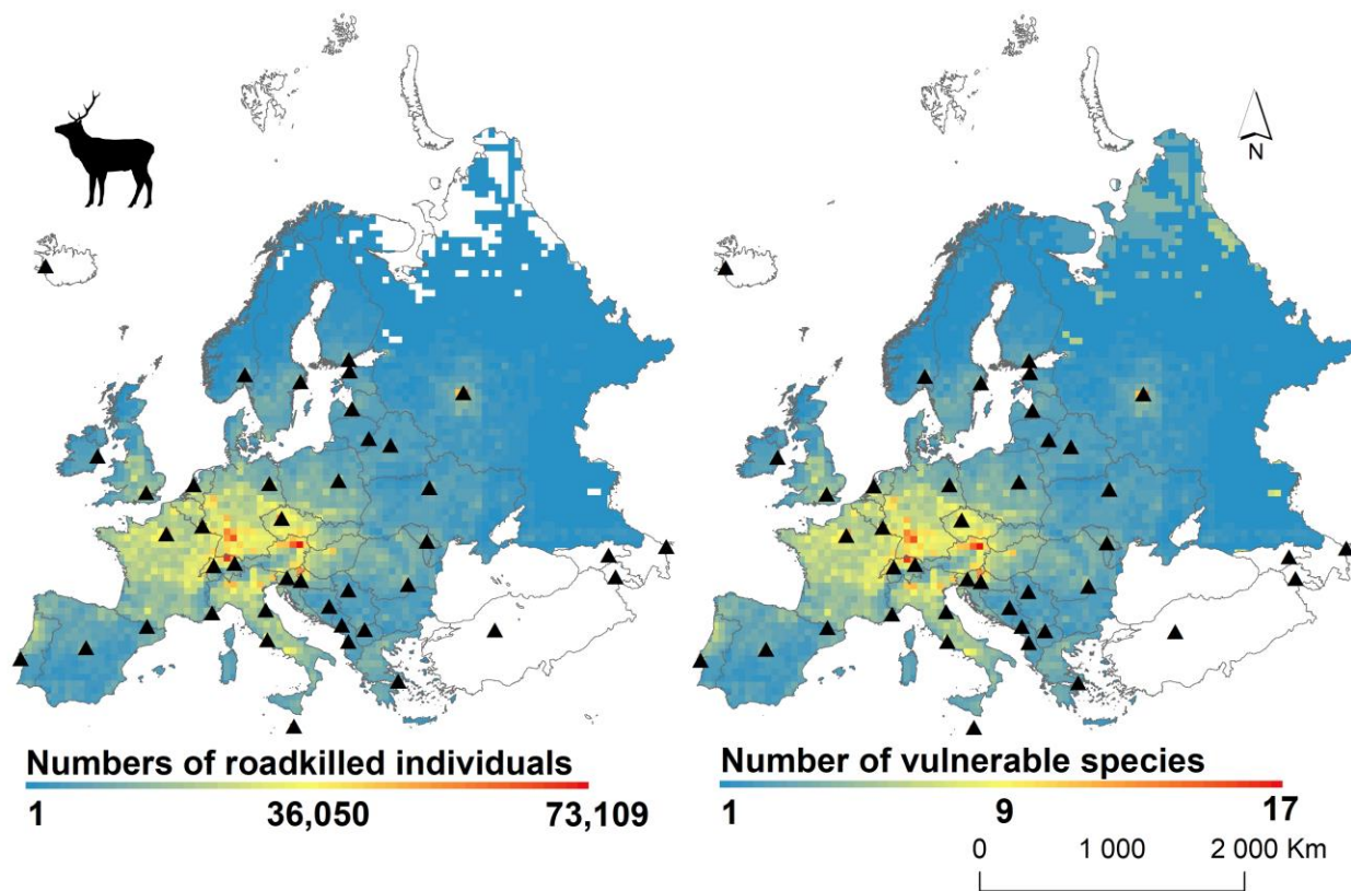
Figure 3 – Cumulative predicted number of mammals killed on roads per year and number of vulnerable mammal species (20th percentile) in each 50-km × 50-km grid cell in Europe. Black triangles mark the locations of major cities.
