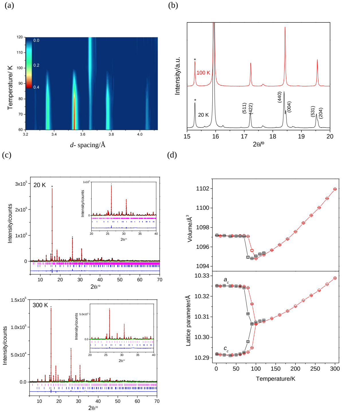
Figure 2. – (a) Powder neutron diffraction data as a function of temperature, over a selected range of d -spacings, showing the appearance of additional reflections; (b) selected synchrotron diffraction data ( \lambda=0.82451 Å), collected below and above the transition, showing the splitting of existing reflections and the appearance of new reflections. Peak from the impurity phase, \text{Cu}_3\text{SbS}_4 , has been labelled with a star. (c) Rietveld refinements using synchrotron X-ray diffraction data collected on \text{Cu}_{12}\text{Sb}_4\text{S}_{13} at 300 and 20 K. Observed, calculated and difference profiles are denoted by black points, a red solid line and a blue line, respectively. The pink and blue reflection markers are for the tetrahedrite phase and the \text{Cu}_3\text{SbS}_4 impurity, respectively. Insets have been added to illustrate the difference between 300 K and low-temperature diffraction patterns. (d) Temperature dependence of the pseudo-cubic lattice parameters, a_c and c_c ; and the unit cell volume of the pseudo-cubic unit cell determined using neutron diffraction data. Error bars lie within the points.
