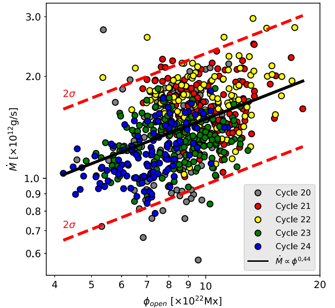
Figure 2. Mass-loss rate, \dot{M} , vs. open magnetic flux, \phi_{\text{open}} , derived from the in situ observations of the OMNI data set. Values are color-coded by sunspot cycle, 20–24. The black line corresponds to the power-law fit of Equation (10). The dashed red lines indicate the 2\sigma bounds given by a log-Gaussian centered on the fit line.
