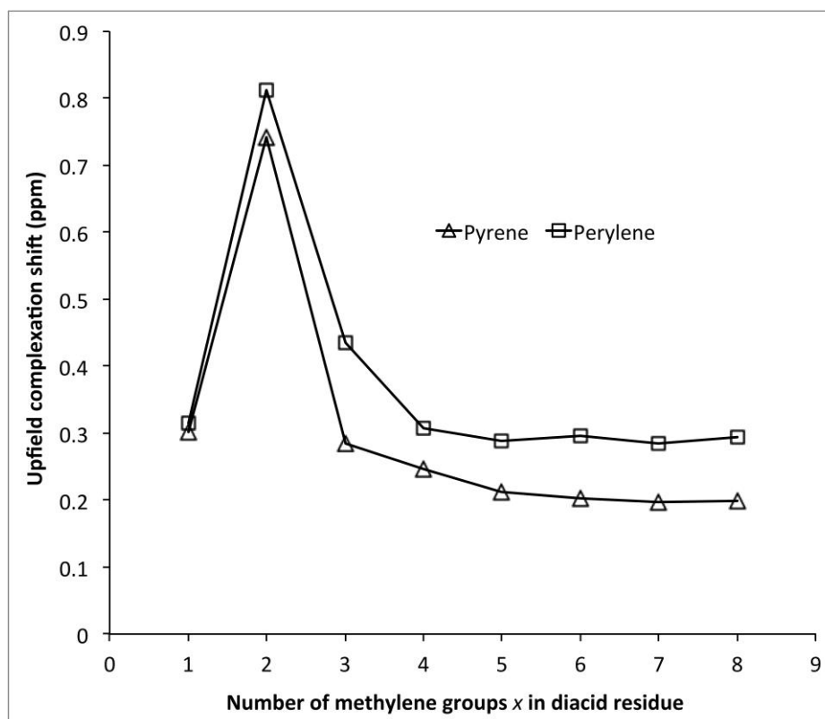
Figure 2. Complexation shifts for NDI-based poly(ester-imide)s 14 – 21 [8 mM in NDI, in CDCl 3 /TFE (6:1 v/v)] in the presence of 2 mol. equiv. per NDI of pyrene- d 10 (△) or perylene- d 12 (□).
