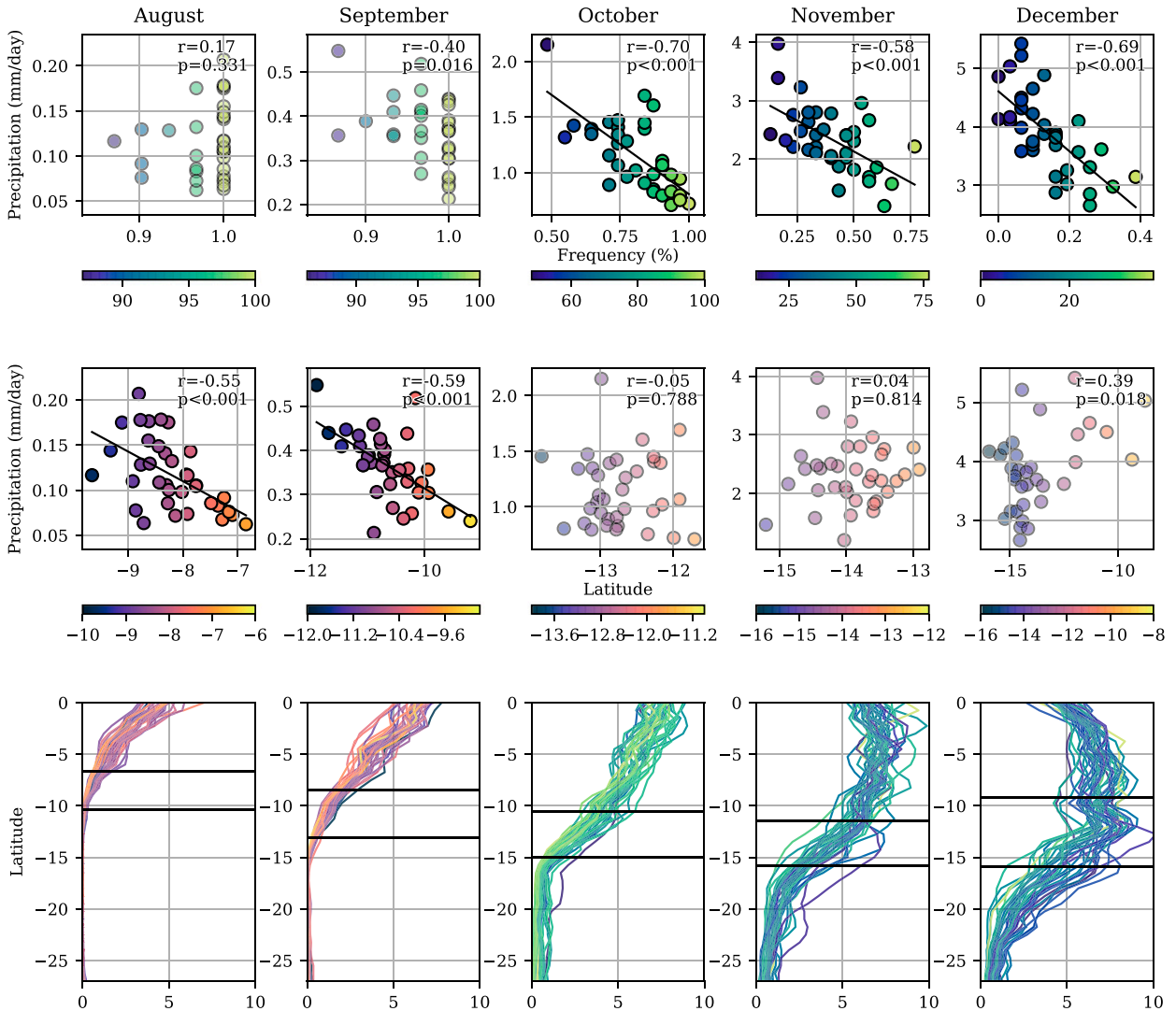
FIG. 10. Interannual rainfall variability due to the CAB. The columns indicate month. (top) Regression of rainfall onto CAB frequency. Rainfall is averaged from CHIRPS between longitudes 15^{\circ} and 25^{\circ}\text{E} and between the 10th-percentile CAB latitude and 25^{\circ}\text{S} . The x axis indicates frequency; the y axis is precipitation ( \text{mm day}^{-1} ). The black line indicates the linear regression of rainfall onto CAB monthly mean CAB latitude when the regression is significant at a p < 0.001 level. Colors also indicate CAB frequency for greater clarity. (middle) As in the top row, but with precipitation regressed on CAB latitude. (bottom) Latitudinal profiles of monthly rainfall for each year between 1981 and 2015. Line color indicates CAB latitude (August and September) and CAB frequency (October–December), using the scales in the first two rows. The x axis is precipitation ( \text{mm day}^{-1} ), and the y axis is latitude. Horizontal black lines represent the 10th- and 90th-percentile latitude of the dryline CAB based on daily data in a given month. Rainfall is averaged between 15^{\circ} and 25^{\circ}\text{E} .
