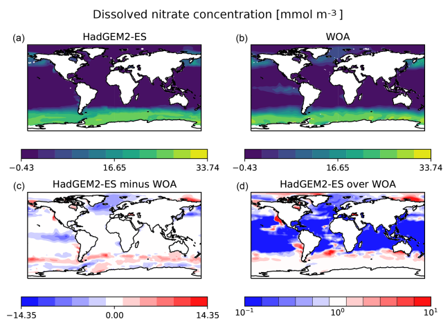
Figure 38. The surface dissolved nitrate concentration in the CMIP5 HadGEM2-ES model compared against the World Ocean Atlas 2013 nitrate. Panels (a) and (b) show the surface fields; (c) and (d) show the difference and the quotient between the two datasets. Produced with recipe_ocean_bgc.yml ; see details in Sect. 3.5.3.
