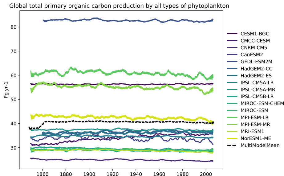
Figure 25. The global total integrated primary production from phytoplankton for a range of CMIP5 models in the historical experiment in the r1i1p1 ensemble member, with a 6-year moving average smoothing function. The multi-model mean is shown as a dashed line. Produced with recipe_ocean_scalar_fields.yml described in Sect. 3.3.1.
