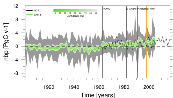
Figure 35. Time series plot of the global land–atmosphere \text{CO}_2 flux ( \text{nbp} ) for CMIP5 models compared to observational estimates from GCP (Le Quéré et al., 2018) (black line). Grey shading represents the range of the CMIP5 models; green shading shows the confidence interval evaluated from the CMIP5 ensemble standard deviation assuming a t distribution centred at the multi-model mean (white line). Vertical lines indicate volcanic eruptions (grey) and El Niño events (orange). Similar to Fig. 5 of Anav et al. (2013) and produced with recipe_anav13jclim.yml ; see details in Sect. 3.5.1.
