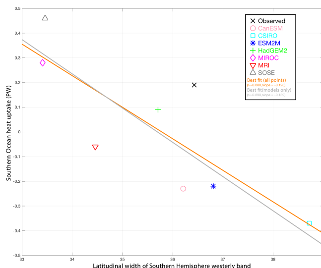
Figure 28. Scatter plot of the width of the Southern Hemisphere westerly wind band (in degrees of latitude) against the annual-mean integrated heat uptake south of 30°S (in petawatts, PW – negative uptake is heat lost from the ocean), along with the “best fit” linear relationship for the models and observations shown. Enhanced from figure produced by recipe_russell18jgr.yml ; see Sect. 3.3.2. For further discussion of this figure, see the original in Russell et al. (2018). The calculation of the “observed” heat flux into the Southern Ocean is described in the text. The correlation is significant above the 98 % level based on a simple t test.
