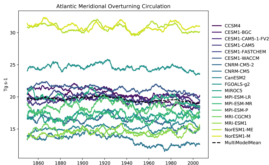
Figure 22. The Atlantic Meridional Overturning Circulation (AMOC) in several CMIP5 models, in the historical experiment, and in the rlilpl ensemble member, with a 6-year moving average smoothing function. The multi-model mean is shown as a dashed line. The AMOC indicates the strength of the northbound current and this current transfers heat from tropical water to the North Atlantic. Produced with recipe_ocean_amoc.yml described in Sect. 3.3.1.
