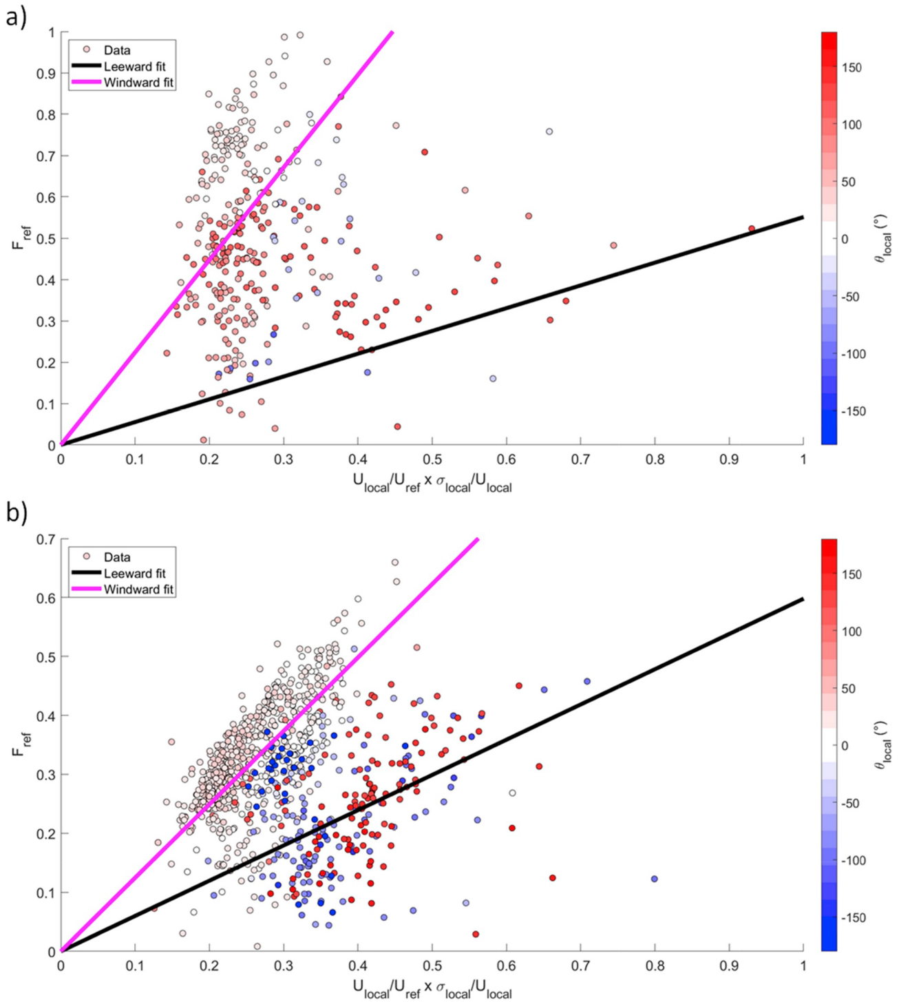
Fig. 9. As Fig. 7, but with \left(\frac{U_{local}}{U_{ref}} \times \frac{\sigma_{local}}{U_{local}}\right) .
