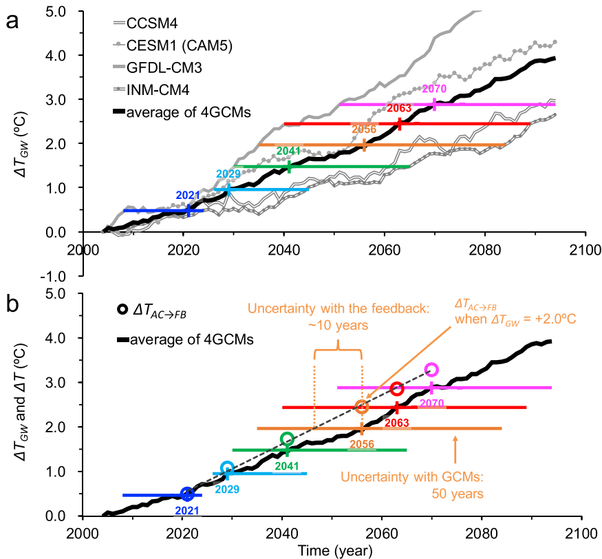
Fig. 4 Changes in August mean surface air temperature for Japan. a Projected increase compared to 2000s (decadal running averages) for four global climate models (CCSM4, CESM1 (CAM5), GFDL-CM3 and INM-CM4; for references, see 'Methods') and the average \Delta T_{GW} (black line) for four GCMs assuming the RCP8.5 scenario (see text for more details). b Time series of \Delta T_{GW} (thick black line) and \Delta T_{AC \rightarrow FB} (circles) with maximum uncertainties (colour lines) of four GCMs and linear approximation of \Delta T_{AC \rightarrow FB} (dashed black line). Values are averaged for three urban categories: commercial and office buildings, fireproof apartments, and wooden detached dwellings
