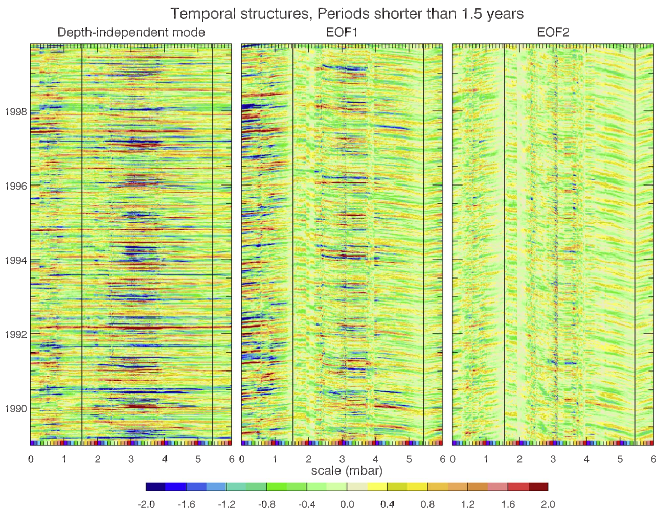
Fig. 12. Hovmöller plots showing the temporal variations in the three vertical (cross-slope) modes as a function of distance along the continental slope and time, after filtering to pass periods shorter than 1.5 years. Linear trend, annual, and semiannual cycles were removed at an earlier stage.
