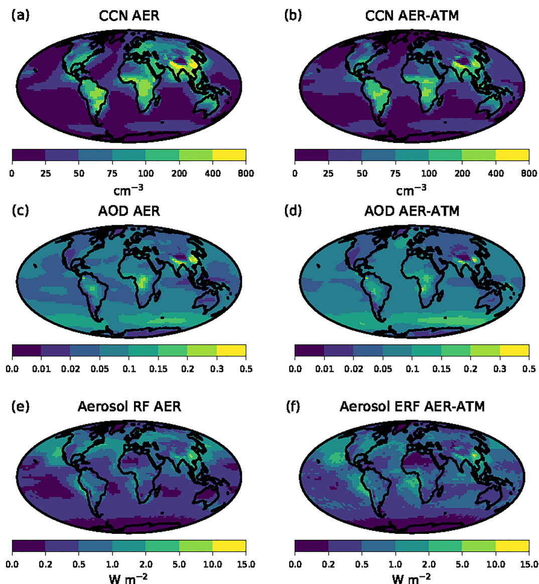
Figure 4. Emulator standard deviations corresponding to the quantities presented in Figure 3.
