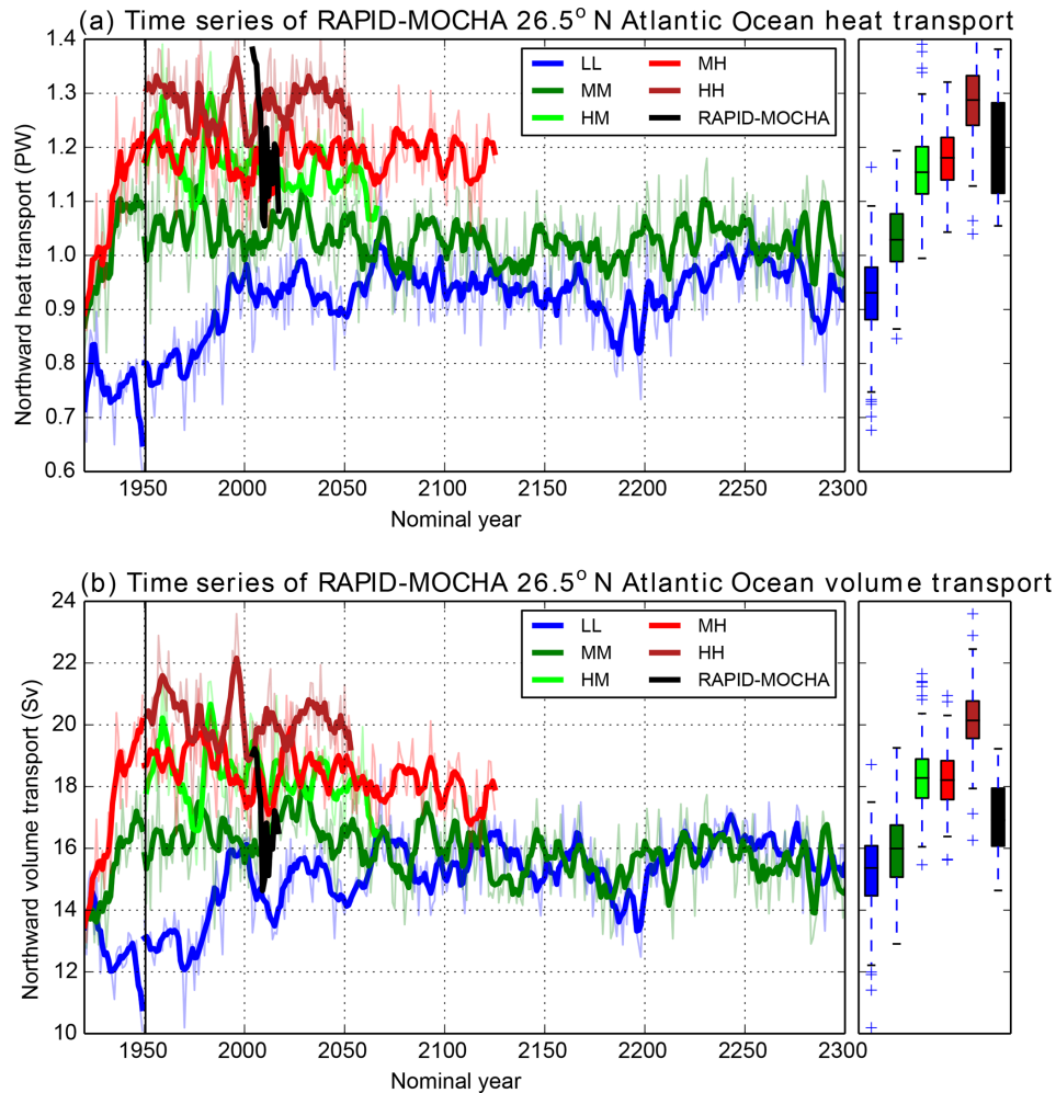
Figure 14. (a) Time series of annual mean (January–December) Atlantic northward ocean heat transport at 26.5^\circ N calculated consistently with the RAPID-MOCHA array using the RapidMoc code (C. D. Roberts, 2017). (b) As above but for volume transport, i.e. the Atlantic meridional overturning circulation at 26.5^\circ N and 1000 m depth, with net transport across sections subtracted. Different model resolutions over the spinup-1950 and control-1950 simulations are shown together with the RAPID-MOCHA observations in black. The thick line shows a 5-year running mean of the annual values (thinner lines). A box-and-whisker plot on the right (using the control-1950 data) shows the lower to upper quartile range as the coloured box; the median (black line within that box) and the whiskers show the range of the data (excluding flier points shown by the + symbol).
