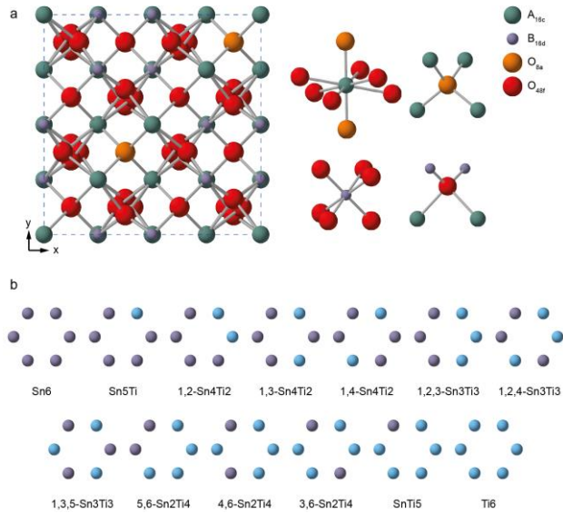
Figure 1. (a) Structure of a typical A_2B_2O_7 pyrochlore, with expansions of the local environments of the Wyckoff 16c (A), 16d (B), 8a and 48f (O) sites. (b) Possible arrangements of Sn and Ti on the six NNN B sites that surround the pyrochlore A and B sites. See the Supporting Information for the numbering scheme used.
