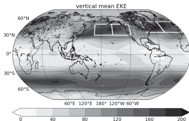
FIGURE 1 Vertically averaged annual mean EKE (in \text{m}^2 \cdot \text{s}^{-2} ), which shows two localised storm tracks in the NH and a more zonally homogeneous Southern Hemisphere storm track. The white boxes show the upstream and downstream regions of the Pacific and Atlantic storm tracks as analysed in this article
