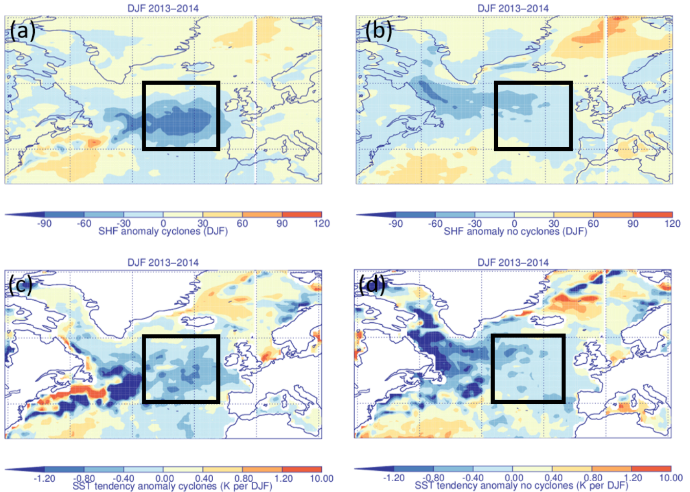
Figure 12. 2013–2014 anomalous Q_N associated with (a) both cyclones and the environmental flow and (b) the environmental flow. 2013–2014 anomalous \Delta\text{SST} due to anomalous Q_N , MLD and entrainment associated with (c) both cyclones and the environmental flow and (d) the environmental flow.
