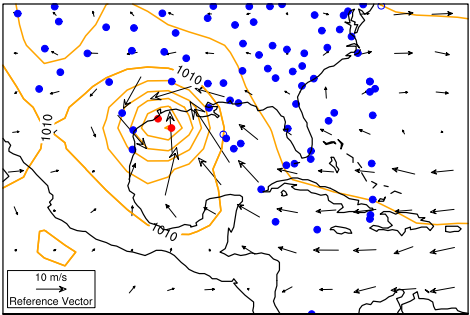
(c) ERA-20C
