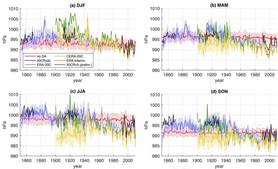
FIGURE 17 Time series of seasonal sea level pressure poleward of 60°S from 20CRv2c (blue), ERA-20C (green), CERA-20C (gold), ERA-Interim (orange), a non-assimilating model run using the 20CRv2c system (red), and preliminary 20CRv3 data without confidence intervals (black). Shading represents one ensemble standard deviation when available.
