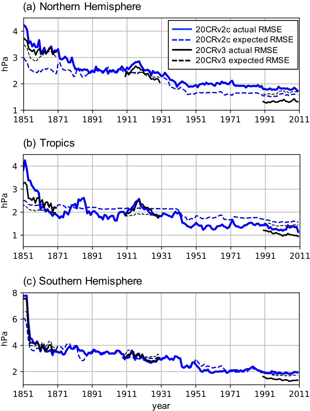
FIGURE 12 Time series of actual (solid) and expected (dashed) annual first-guess RMS errors for observations assimilated in 20CRv2c (blue) and 20CRv3 (black) averaged over (a) the Northern Hemisphere (20°N to 90°N), (b) the tropics (20°S to 20°N), and (c) the Southern Hemisphere (90°S to 20°S).
