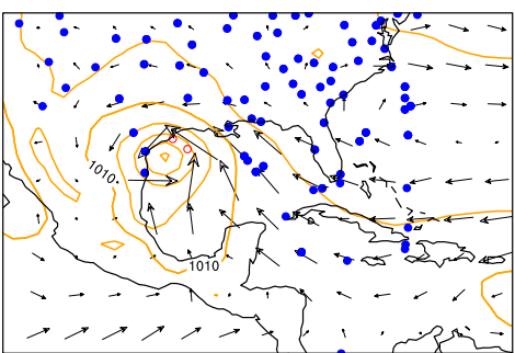
(c) ERA-20C
