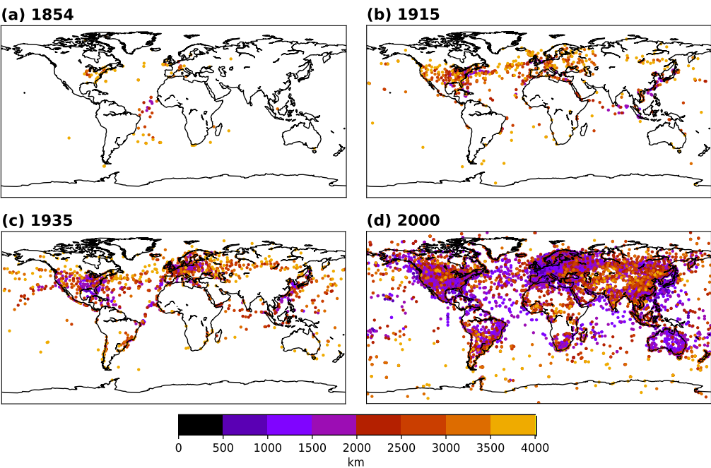
FIGURE 11 Localization values (km) for all observations assimilated in 20CRv3 at 1200 UTC on 1 June for the years (a) 1854, (b) 1915, (c) 1935, and (d) 2000. Note that comparable plots for 20CRv2c would consist entirely of light orange circles (localization value of 4000 km).
