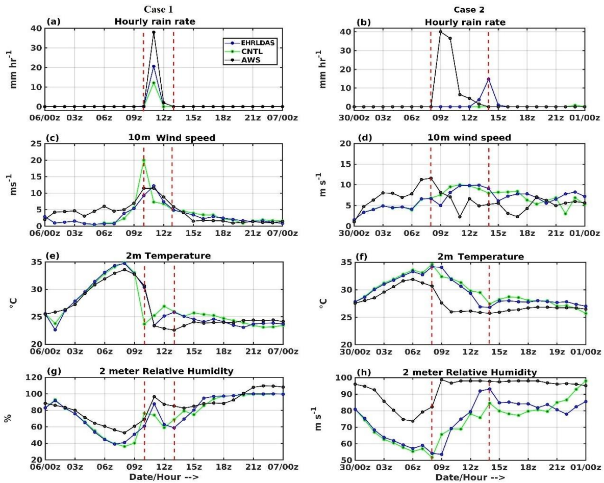
Figure 4. Time series of surface parameters (rain rate ( \text{mm hr}^{-1} ), 10m wind speed ( \text{m s}^{-1} ), 2 metre temperature ( ^{\circ}\text{C} ) and 2 metre relative humidity (%)) for the two thunderstorm cases i.e. (a, c, e, and g) for Case 1 and (b, d, f, h) for Case 2 from CNTL, EHRLDAS and AWS data. Vertical red lines representing the event duration over Argul ( 85.70^{\circ}\text{E} , 20.17^{\circ}\text{N} ).
