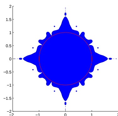
(vi) \bigcup_{\substack{p \in S \\ \deg(p) = 12}} p^{-1}(\mathbb{D})
