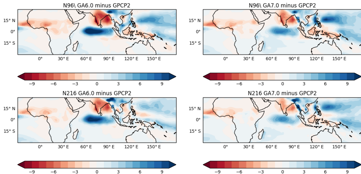
Figure 18. JJA precipitation rate biases versus GPCP over the Indian Ocean and the maritime continent ( \text{mm day}^{-1} ) from 27-year N96 and N216 atmosphere/land-only climate simulations of GA6.0 and GA7.0. The layout is the same as in Fig. 17.
