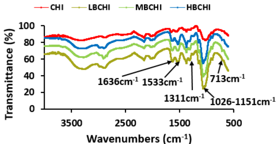
Fig. 3. FT-IR spectra of chitosan and boronated chitosan with distinct peak at 1311\text{ cm}^{-1} indicative of \text{B(OH)}_2 groups; absorption bands at 713 and 1533\text{ cm}^{-1} depicted p-substituted benzene and absorption band confirming \text{NH-CO-} linkage between chitosan and boronate groups evident at 1636\text{ cm}^{-1} .
