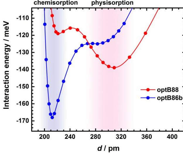
Figure 3. Interaction energies (per BN formula unit) as functions of the average separation d between the Ni substrate and the h -BN monolayer, as calculated for the N( top )-B( fcc ) configuration, using the optB88-vdW and optB86b-vdW functionals. The saddle points were located by means of nudged elastic band calculations.
