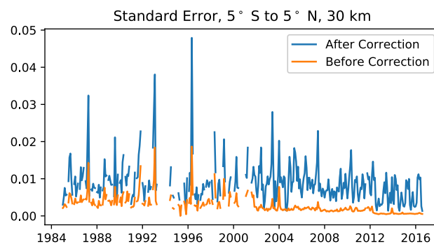
Figure 4.3: Standard errors between 5°S–5°N at 30 km used for the weighted regression applied to the merged SAGE-OSIRIS-OMPS ozone data set both before and after the heteroscedasticity correction. Note how the errors/weights before the correction drop/rise dramatically once OSIRIS (added in 2001) and OMPS (added in 2012) are added as a result of increased sampling of the instruments.
