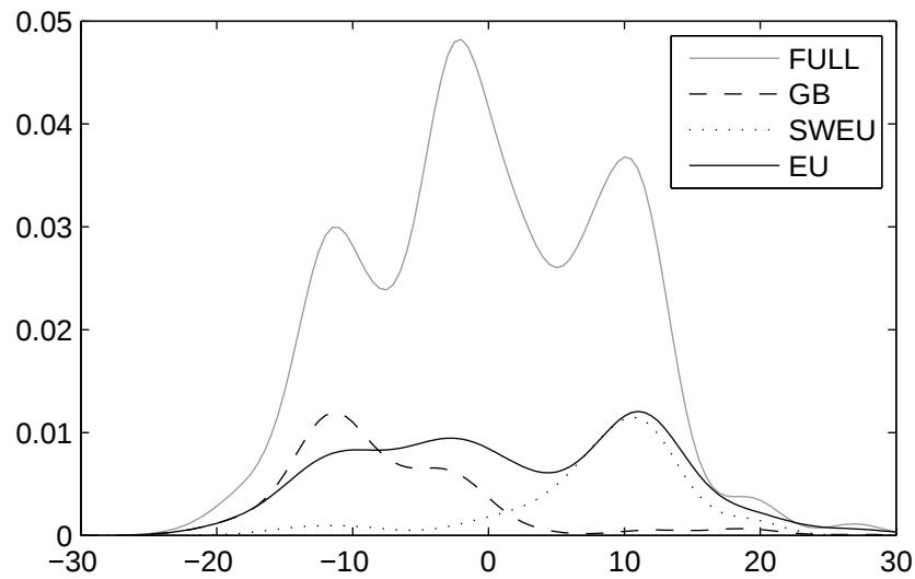
Figure 8. Kernel estimates of the PDF of jet latitude, as in Figure 1, but for days exhibiting blocking over different locations (GB: Greenland Blocking, (53 °N, 50 °W); SWEU: South-west Europe, (41 °N, 15 °W); EU: Europe, (53 °N, 15 °E)). The PDF of the full dataset is shown in grey and the other PDFs have been scaled by the number of days in each set.
