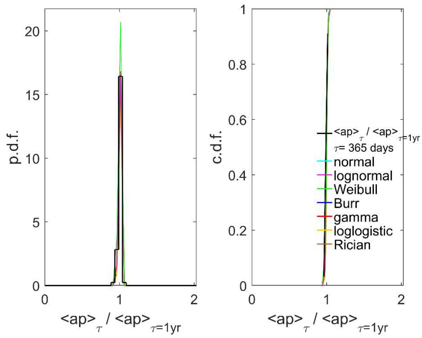
Figure S6. Same as Figure S1 but for an averaging timescale \tau = 1 year
