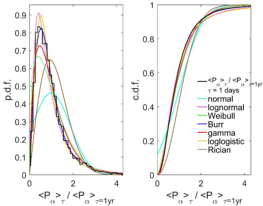
Figure S14. Same as Figure S13 but for an averaging timescale \tau = 1 day.
