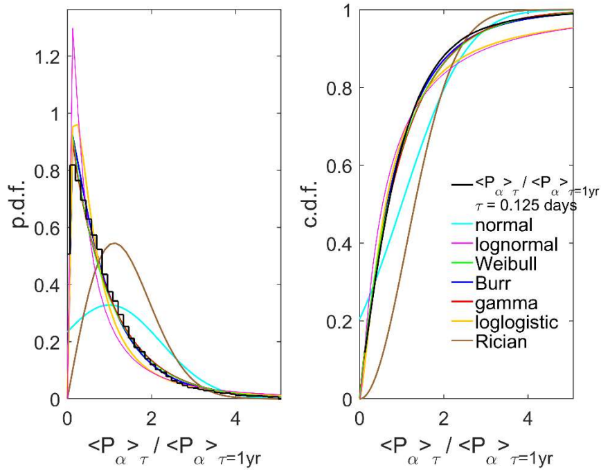
Figure S13. Same as Figure S1 but for the ratio \langle P_{\alpha} \rangle_{\tau} / \langle P_{\alpha} \rangle_{\tau=1\text{yr}} for the estimated power input into the magnetosphere, P_{\alpha} (and for an averaging timescale \tau = 3 hours)
