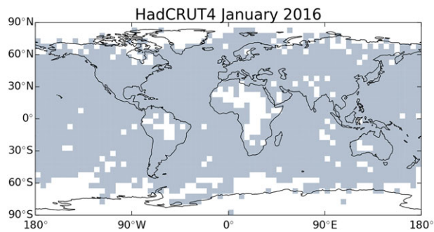
Figure 2. Missing data (white grid cells) in the HadCRUT4 network as of January 2016. Unsampld regions are concentrated in the high latitudes, Africa and South America. HadCRUT4 = Hadley Centre-Climatic Research Unit Version 4.
