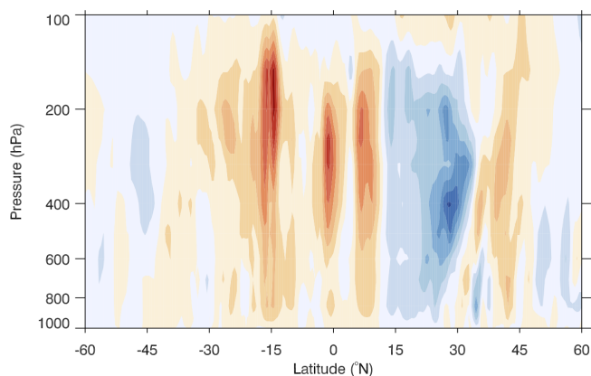
Figure 7. Vertical velocity ( \text{m s}^{-1} ) averaged over the 5^\circ of longitude centred on 140^\circ \text{E} . Positive values indicate ascent.
