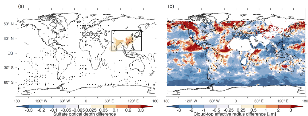
Figure 2. Ensemble mean, (1998–2012) vs. (1979–1993), difference in (a) sulfate optical depth (with the black box indicating the emission region), and (b) cloud-top effective radius. Dots indicate where the response is not significant at the 10 % level, as calculated using a two-tailed Student's t test. Figure 6c shows the agreement of individual ensemble members on the sign of the anomaly in cloud-top effective radius shown in panel (b).
