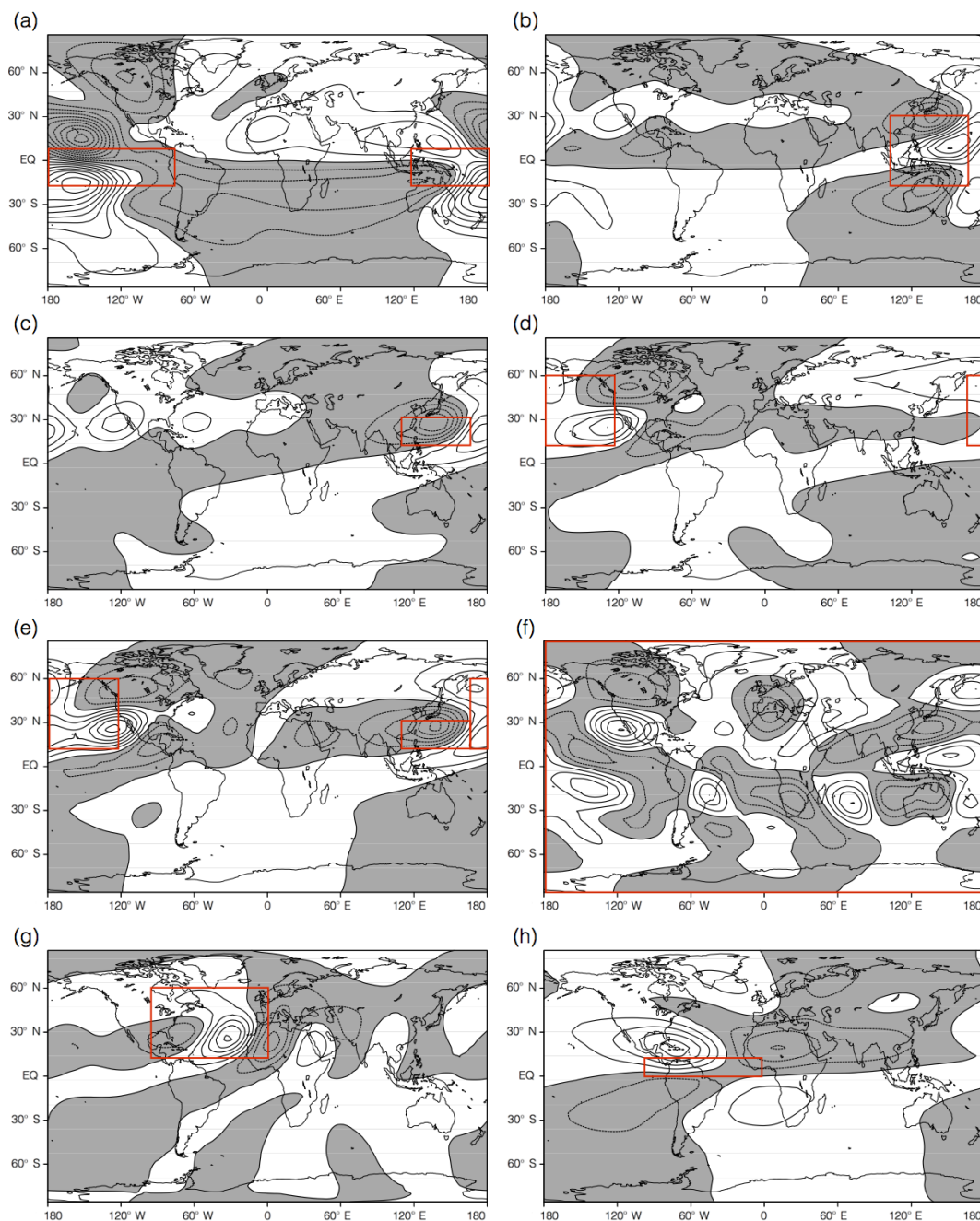
Figure 9. The 250 hPa stationary wave anomaly from LUMA when forced with the HadGEM3-GC2, (1998–2012) vs. (1979–1993), precipitation anomaly (a) from the equatorial Pacific (15° S to 10° N, 120° E to 75° W); (b) downstream of China and Indonesia (15° S to 30° N, 100 to 160° E); (c) downstream of China (15° S to 30° N, 110 to 160° E); (d) the northern North Pacific (15 to 60° N, 160 to 240° E); (e) the sum of regions (c) and (d); (f) the whole globe; (g) the North Atlantic (15 to 60° N, 0 to 90° W), and (h) the tropical North Atlantic (0 to 15° N, 0 to 90° W). Grey shading and dashed contours indicate negative anomalies, white shading and solid contours indicate positive anomalies. Red boxes indicate the location of the precipitation anomaly.
