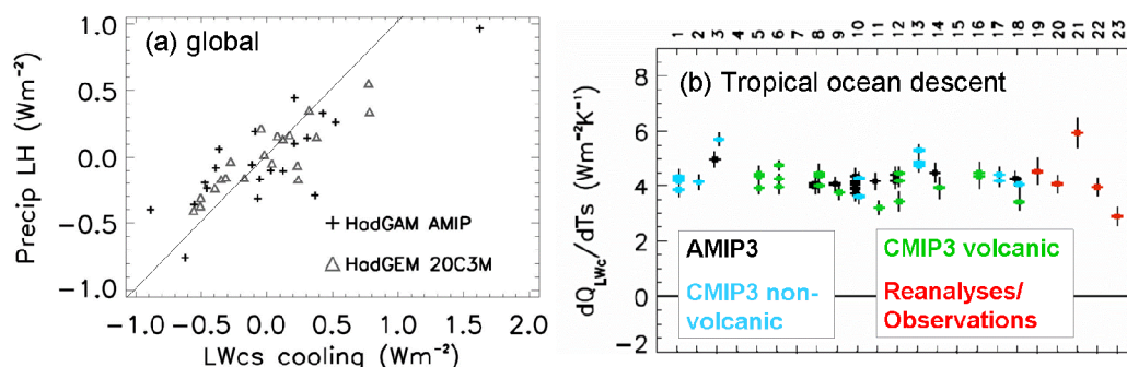
However, by combining the surface and top of atmosphere clear-sky radiative fluxes, the clear-sky longwave radiative cooling of the atmosphere ( Q_{LWC} ) shows surprisingly good agreement between models, reanalyses and observations for much of the period (excluding the CERES observations after 2000, the Pinatubo and the El Chichon volcanic eruptions and the ERA40 data around January 1986, Fig. 1e). This is partly explained by the fact that humidity errors in the reanalyses produce compensating biases in the clear-sky longwave radiative cooling of the atmosphere at the surface and at the top of atmosphere (Allan, 2006).
