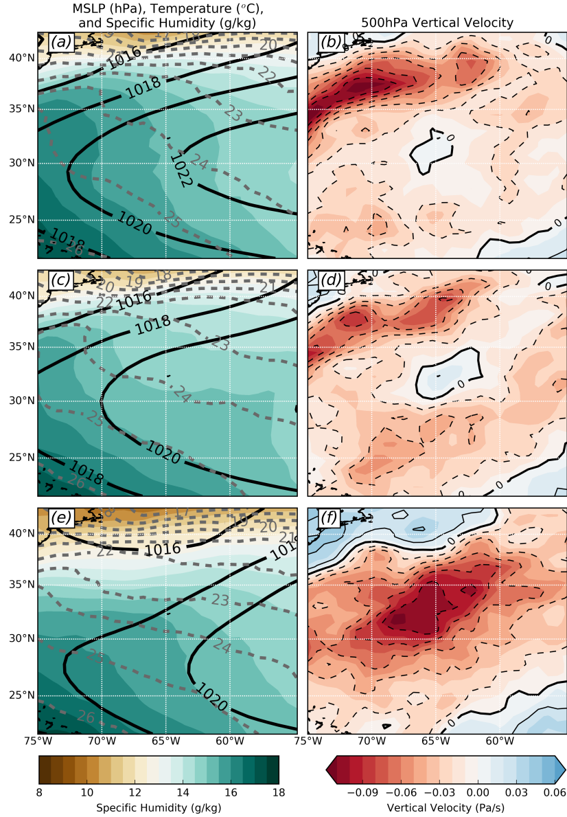
FIG. 5. JJA, 2012-2016 ERA-interim reanalysis composites centered on Bermuda. (a) and (b) are composites for Cloud Trails, (c) and (d) are composites for Non-Trails, and (e) and (f) are composites for Obscured. The left-hand column shows the mean sea-level pressure in hPa (solid black contours), 1000-hPa temperature in ^{\circ}\text{C} (dashed grey contours), and 1000-hPa specific humidity in \text{g kg}^{-1} (shading). The right-hand column shows the 500-hPa vertical velocity in \text{Pa s}^{-1} , ascent and subsidence are shown in dashed and solid contours respectively.
