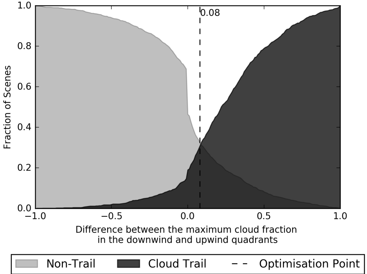
Fig. A2. Cumulative distribution function of the difference in maximum downwind and upwind cloud fraction, \delta F , for CT scenes compared to \delta F for NT scenes. The difference at the intersection of these two distributions, 0.08, is taken as the value of our parameter \beta .
