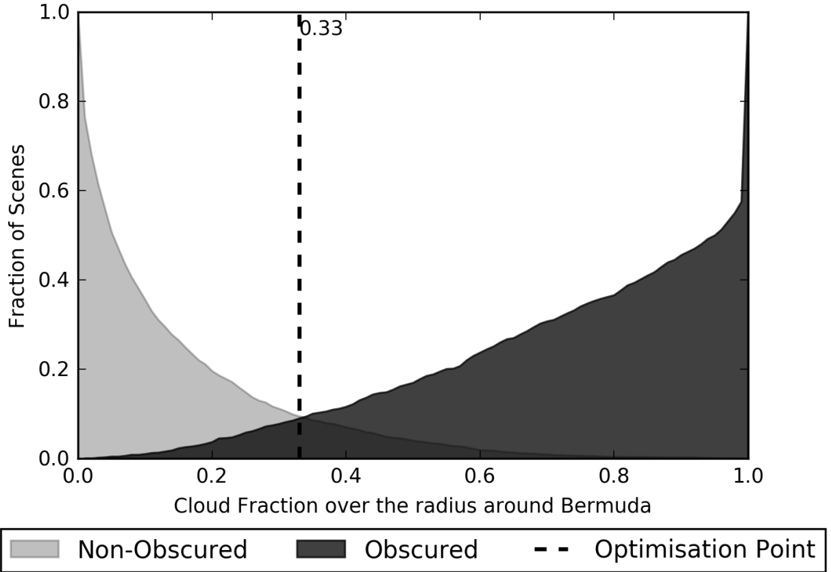
Fig. A1. Cumulative distribution function of the cloud fraction for OB scenes and the inverse cumulative distribution function of the cloud fraction for non-OB scenes. The cloud fraction value at the intersection of these two distributions, 0.33, is taken as the value of our parameter \alpha .
