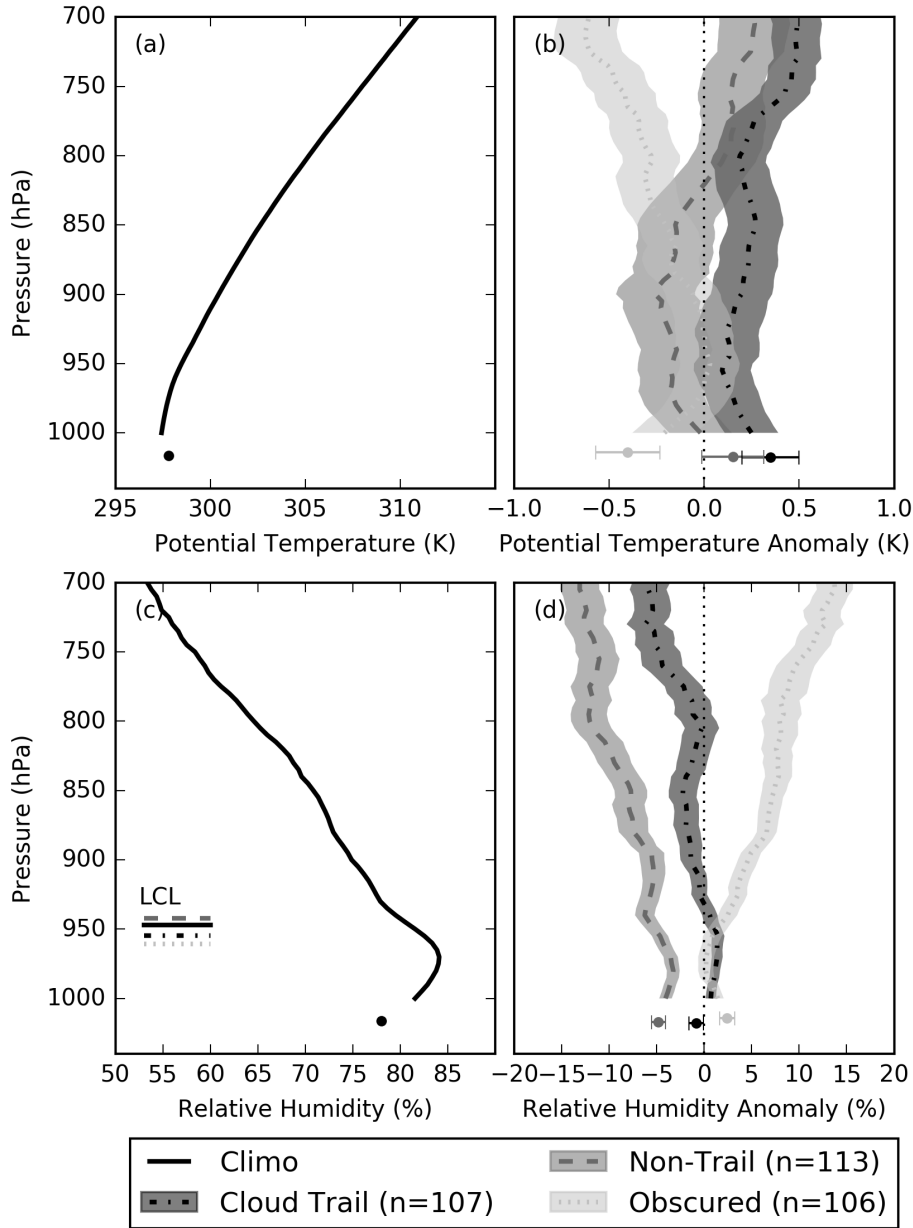
FIG. 4. (a) The climatological potential temperature ( \theta ) profile. The mean surface \theta is marked with a black dot. (b) The composite \theta anomalies for CT (dash-dot line with dark grey shading), NT (dashed line with grey shading), and OB (dotted line with light grey shading). The shaded region represents the uncertainty about the mean anomaly: \pm \frac{\sigma}{\sqrt{N}} . The surface \theta for each classification is shown by dots with the corresponding shade of grey. The range on the surface values is again \pm \frac{\sigma}{\sqrt{n}} . (c) The mean climatological relative humidity profile as in (a). The mean LCL for each classification, and for the climatology are shown as horizontal line segments with corresponding line styles. (d) The composite relative humidity anomalies. Composites are for the 0900 LT radiosondes for JJA in 2012-2016. In each case, only data between the surface and 700-hPa are shown. LCL pressures are calculated using the temperature and dew point of the lowest altitude reported by the radiosonde and equations 5 and 6.
