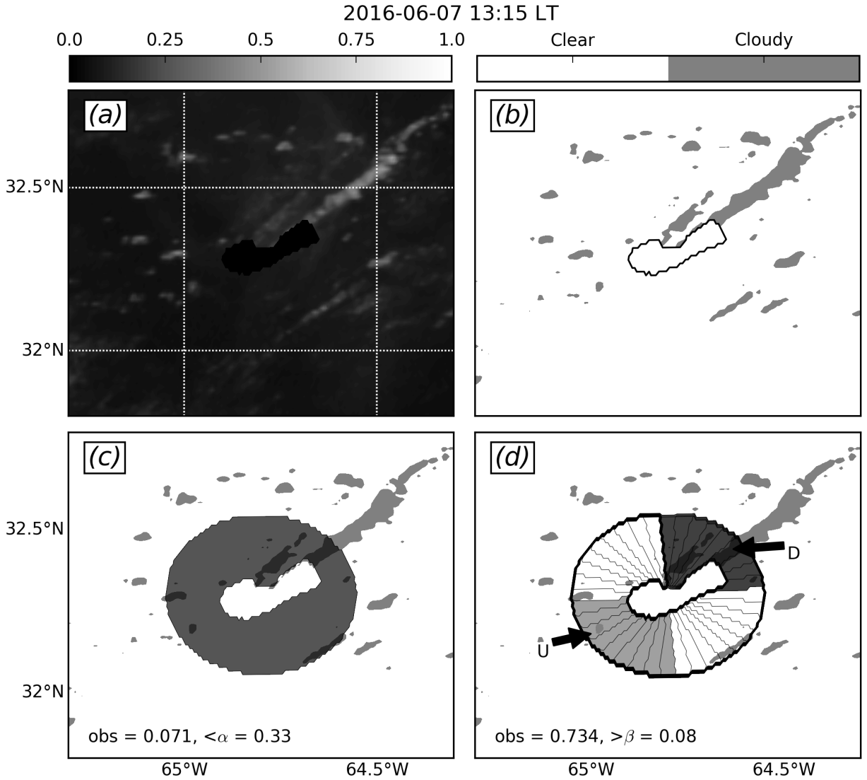
FIG. 2. A walkthrough of the steps taken to classify each scene. (a) GOES-13 visible-channel satellite imagery. (b) Cloud mask applied to (a), cloudy pixels are shown in grey. (c) The cloud fraction in the circular area centered on 32.3°N, 64.8°W with a radius of 0.25° (dark grey shaded region) is used to determine if the scene is OB. In this example, the cloud fraction is 0.071 which is less than \alpha = 0.33 and so the scene is non-OB. (d) Since the scene is non-OB, the same circular area from (c) is split into 10° wide sectors, thirty-six in total. The 10 m wind direction at TXKF is used to find the upwind and downwind quadrant (i.e. nine sectors in each direction). The cloud fraction is calculated for each sector of the upwind quadrant (light grey) and the downwind quadrant (dark grey). The difference between the maximum downwind cloud fraction (arrow marked with 'D') and the maximum upwind cloud fraction (arrow marked 'U') has to be greater than \beta = 0.08 for the scene to be classified as CT.
