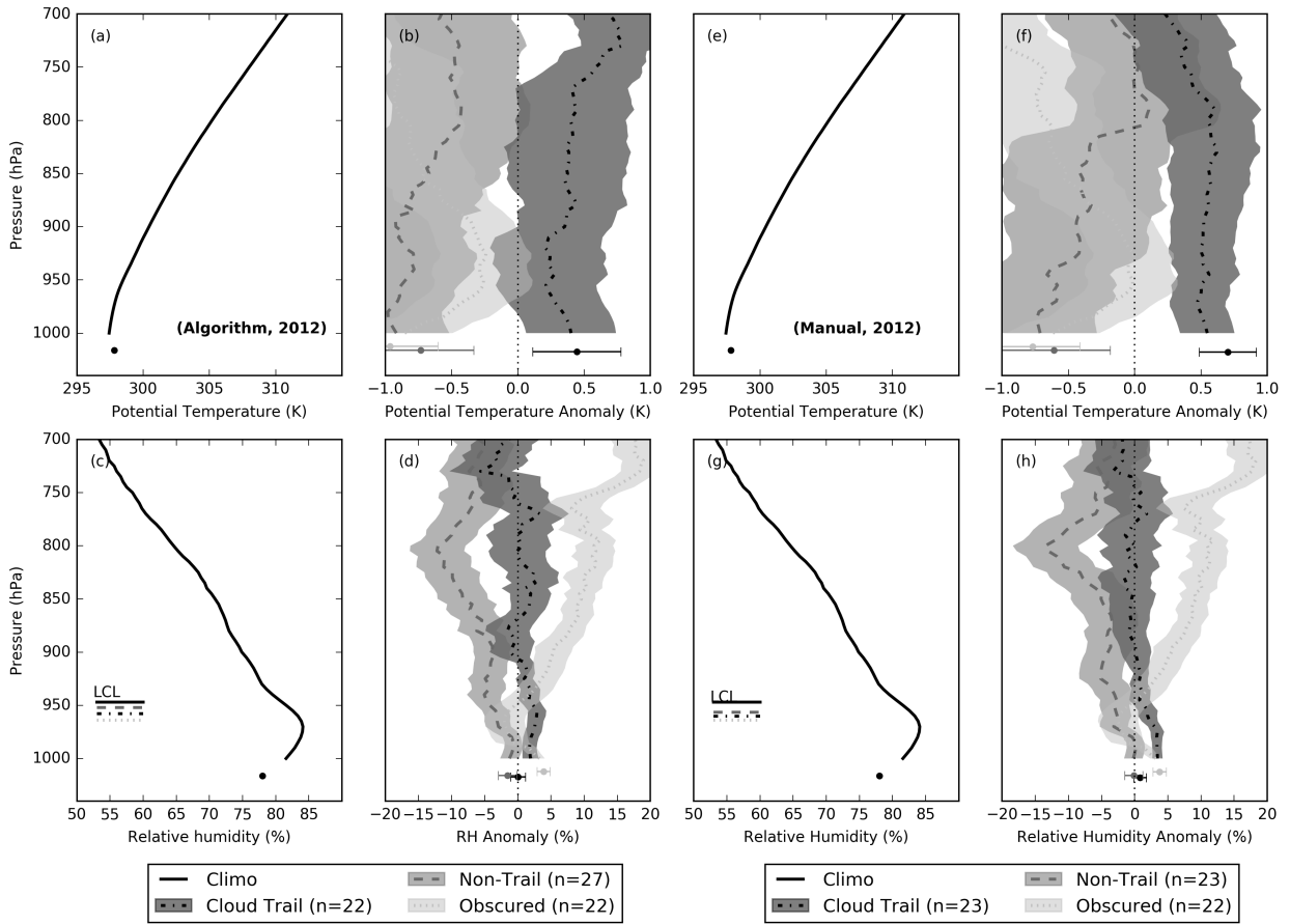
Fig. A5. As in Figure 4, but for the classifications for May through October 2012. Note that these are anomalies with respect to the 2012-2016 JJA climatology. These profiles are made for the algorithm classifications on the left and the manual classifications on the right.
