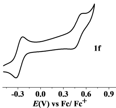
Figure S2. The curtailed two-anodic-step cyclic voltammogram (CV) of 1f in CH 2 Cl 2 / n -Bu 4 NPF 6 at \nu = 50 \text{ mV s}^{-1} .
