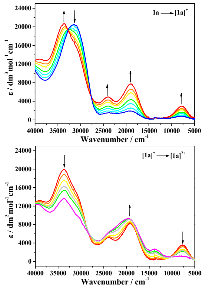
Figure 3. Changes in UV-vis-NIR absorption spectra recorded during the oxidation of complex 1a to [1a]^+ (top) and [1a]^{2+} (bottom) in CH_2Cl_2/10^{-1} M n-Bu_4NPF_6 at 298 K within an OTTLE cell.
