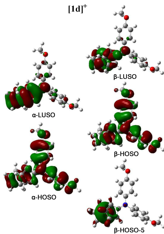
Figure S9. Spin orbitals involved in the major electronic excitations of [1d]^+ . B3LYP /6-31G* (Fe: Lan12DZ) /CPCM /CH 2 Cl 2 .
