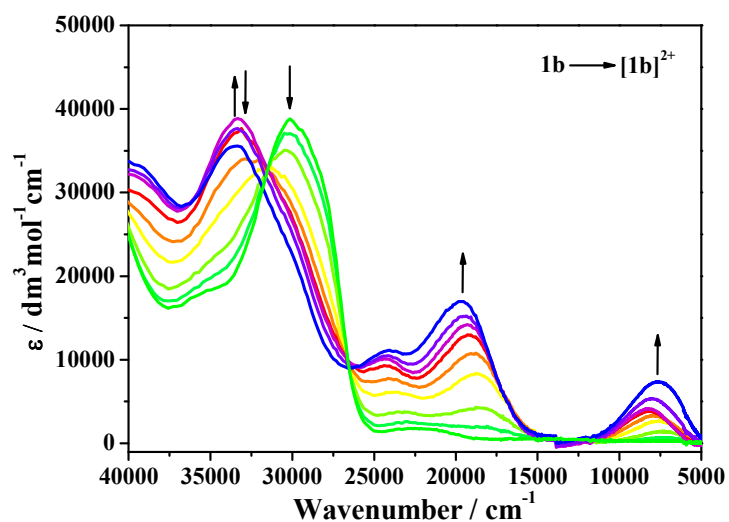
Figure S3. Changes in UV-vis-NIR absorption spectra recorded during the oxidation of complex 1b to [1b] 2+ in CH 2 Cl 2 / 10^{-1} M n -Bu 4 NPF 6 at 298 K within an OTTLE cell. The intermediate absorption of [1b] + is poorly resolved due to pronounced redox disproportionation of the monocation.
