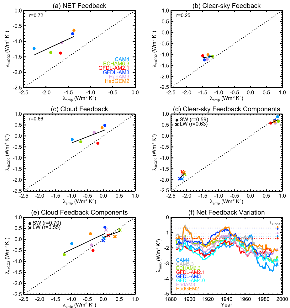
Figure 2. Relationship between the feedback parameter evaluated by regression of dN against dT over the historical period (1871–2010) in amip-piForcing ( \lambda_{\text{amip}} ) and 150 years of abrupt-4xCO 2 ( \lambda_{4\text{xCO}_2} ) for (a) NET radiative feedback, (b) clear-sky component, (c) CRE component, (d) LW and SW clear-sky components, and (e) LW and SW CRE components. (f) Time series of \lambda_{\text{amip}} for individual AGCMs evaluated by linear regression of dN against dT in a sliding 30-year window in the amip-piForcing experiments, the year represents the center of the window. Colored circles in (f) with horizontal lines show the feedback parameter values from abrupt-4xCO 2 . LW = longwave; SW = shortwave.
