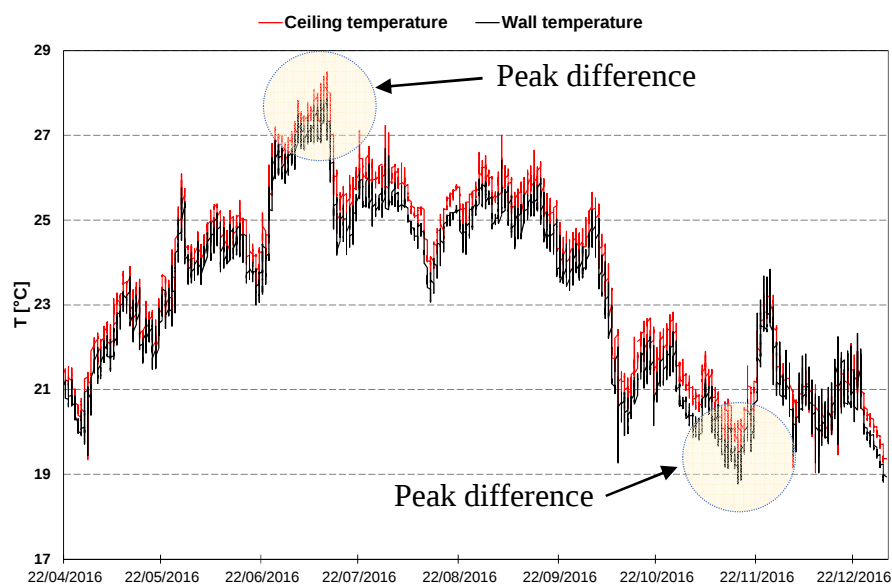
Figure 12. Ceiling and wall temperature trends during the measurement campaign (the highlighted zones identify major deviations)
