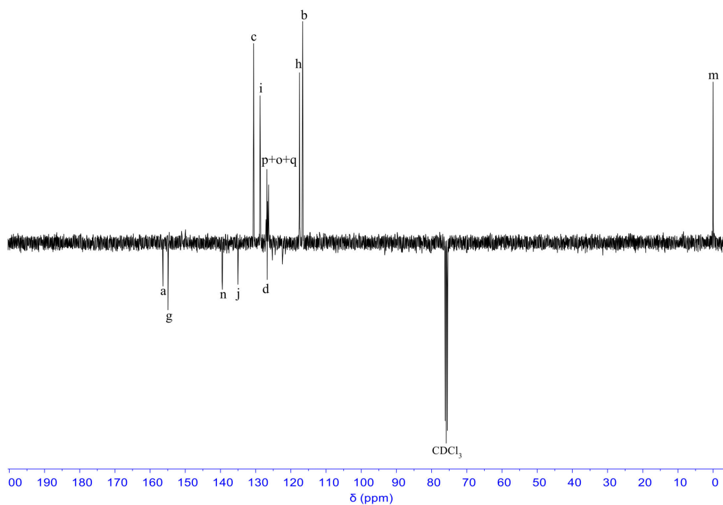
Figure S49. ^{13}\text{C} NMR (DEPT-135) spectrum of poly[(trifluoromethyl)(trimethylsilyl)ether] 11 (100 MHz, \text{CDCl}_3 ).
