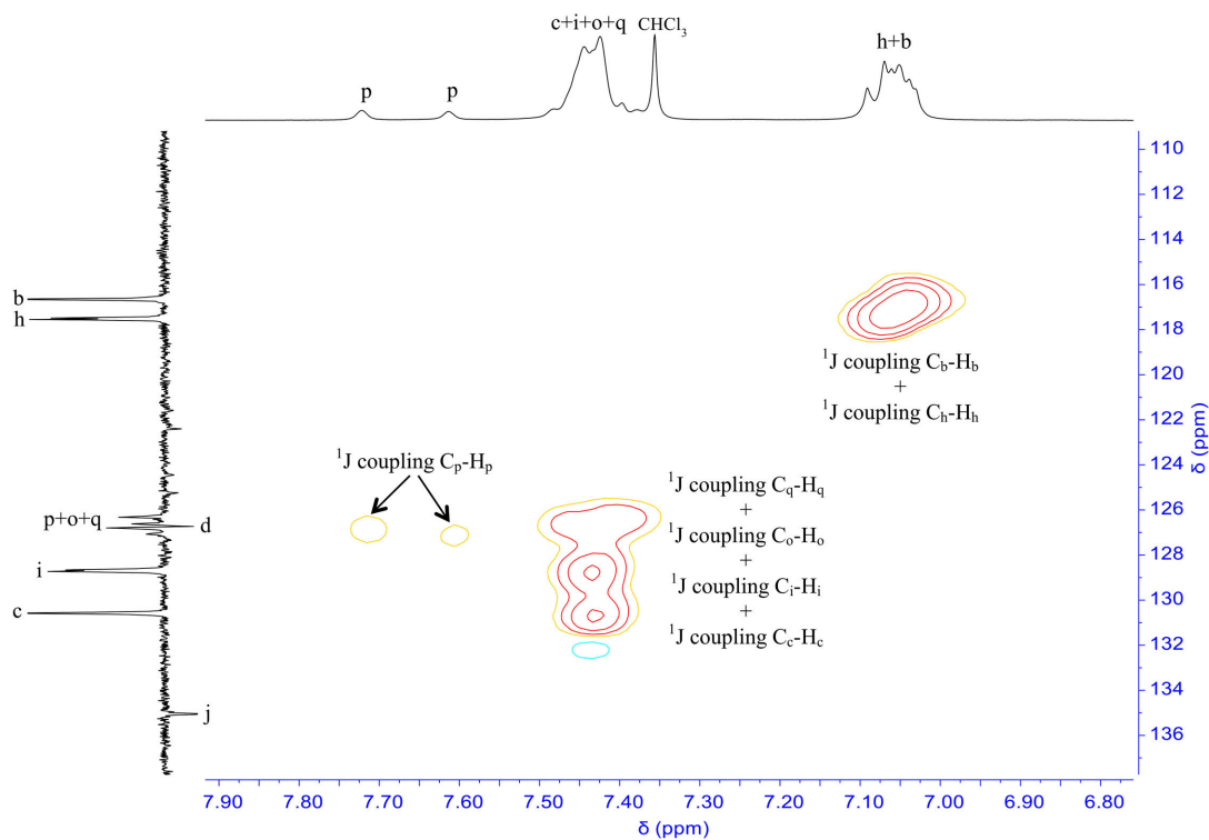
Figure S50. HSQC ( ^1\text{H} - ^{13}\text{C} ) NMR spectrum of poly[(trifluoromethyl)(trimethylsilyl)ether] 11 ( \text{CDCl}_3 ).
