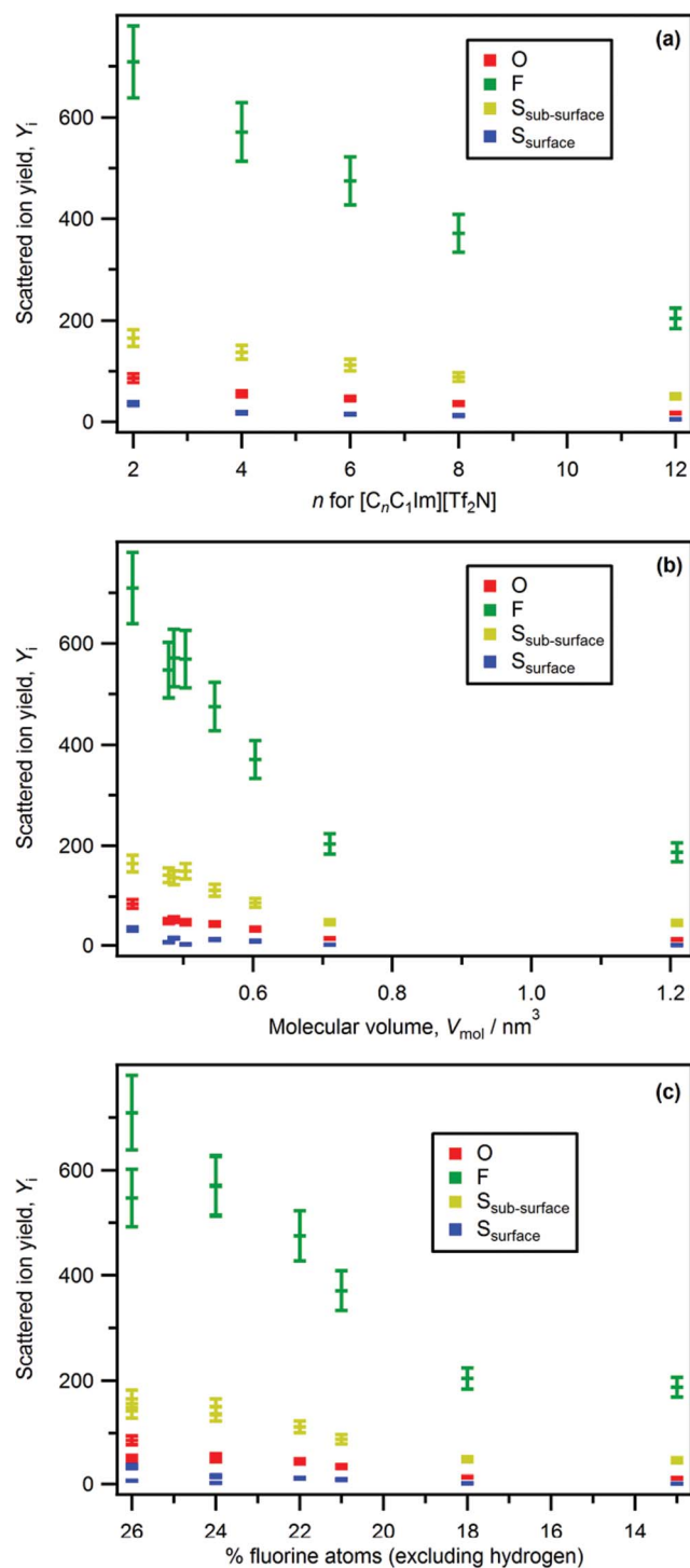
Fig. 8 Scattered ion yield, Y_i , for [\text{C}_n\text{C}_1\text{Im}][\text{TF}_2\text{N}] , [\text{C}_4\text{C}_1\text{Pyr}][\text{TF}_2\text{N}] , [\text{N}_{4,1,1,1}][\text{TF}_2\text{N}] and [\text{P}_{6,6,6,14}][\text{TF}_2\text{N}] vs.: (a) n for [\text{C}_n\text{C}_1\text{Im}][\text{TF}_2\text{N}] , (b) molecular volume, V_{\text{mol}} , (c) percentage of fluorine atoms (excluding hydrogen atoms).
