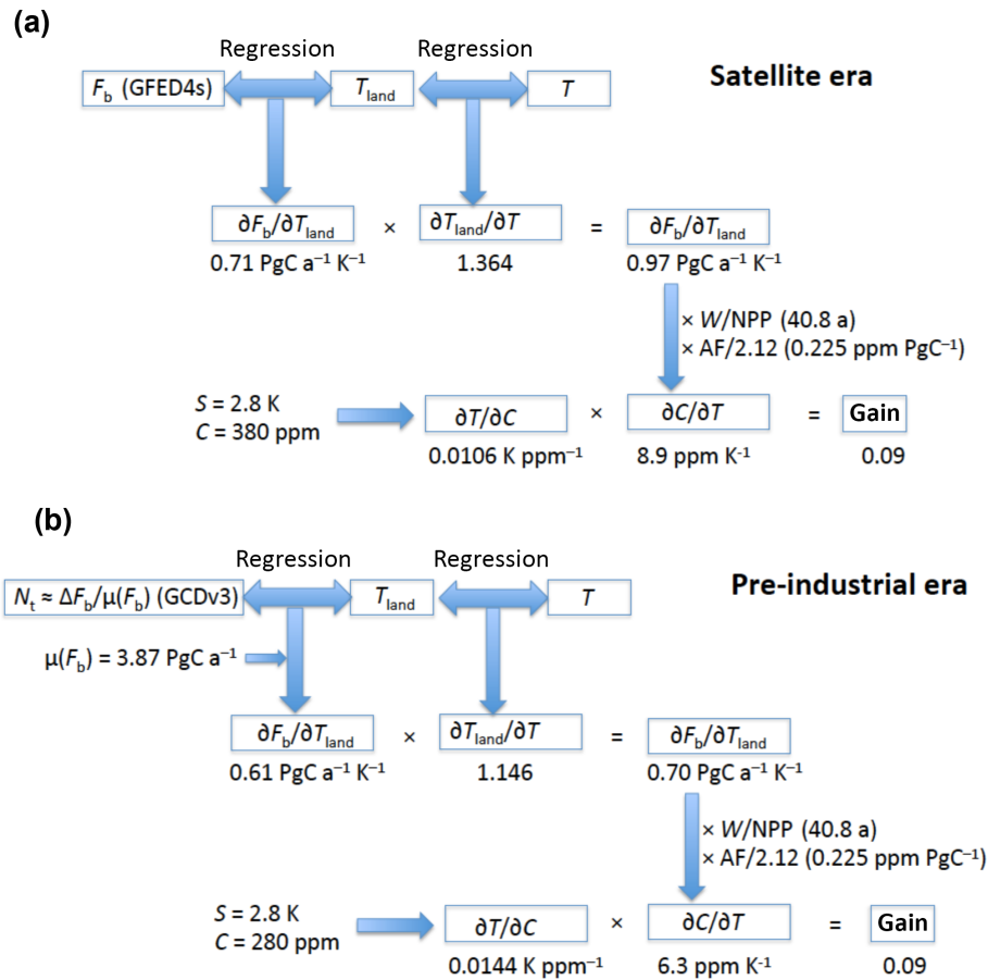
Figure 1. Schematic of the analysis of global fire–temperature relationships for the (a) satellite and (b) pre-industrial eras. F_b : biomass burning flux; T_{\text{land}} : global mean land temperature; T : global mean temperature; W : global land carbon storage; NPP: global net primary production; W/\text{NPP} : residence time of land carbon; AF: airborne fraction; 2.12: conversion factor from ppm to \text{PgC}^{-1} ; S : climate sensitivity; C : atmospheric \text{CO}_2 mole fraction; N_t : normalized anomalies of charcoal data; \Delta F_b : biomass burning flux anomalies; \mu(F_b) : mean biomass burning flux. See text for sources of temperature data.
